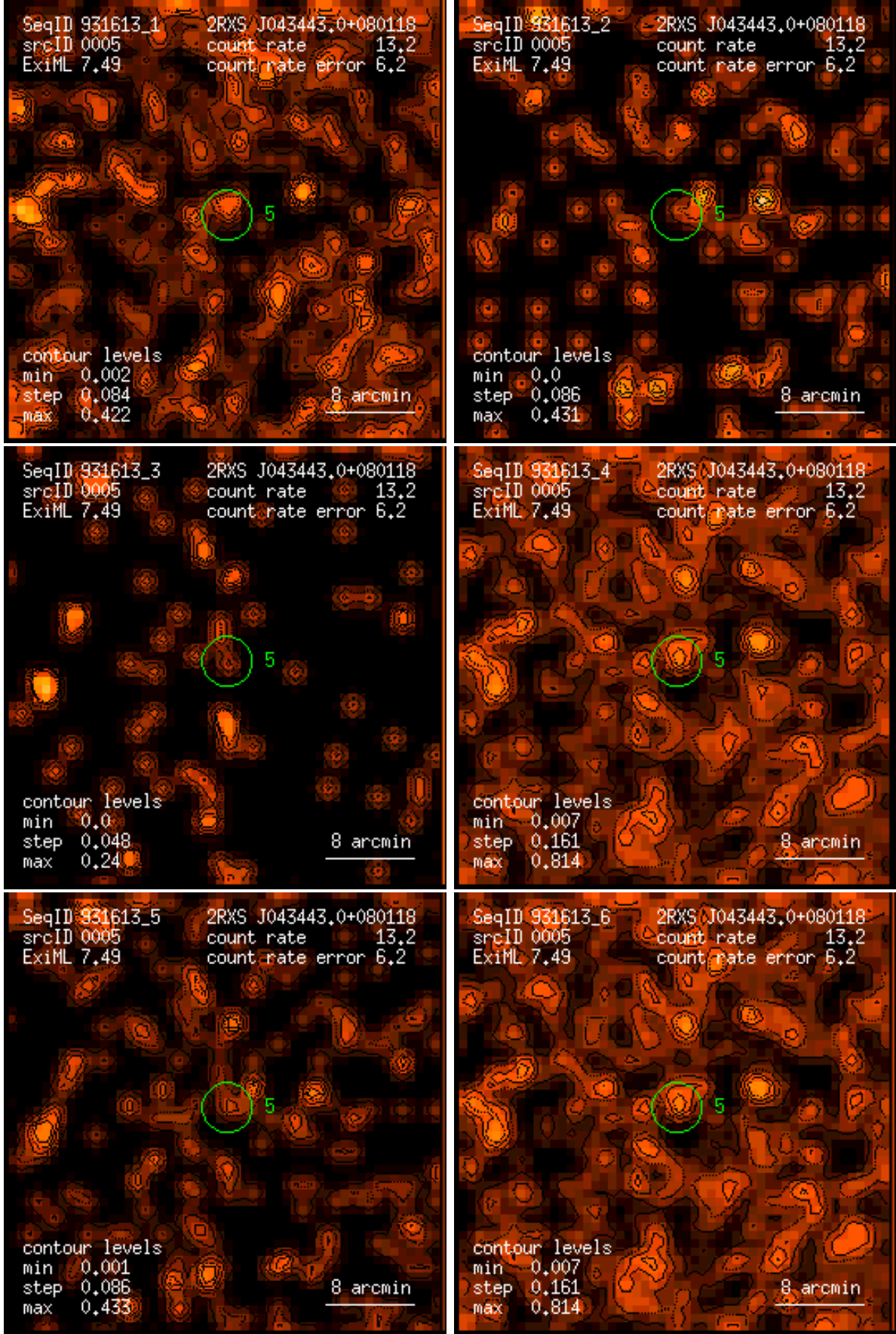
Figure 5: RASS 931613: detection 0005: band rate images, Gaussian filter: (1) PSPC channels 11 – 41, (2) 52 – 90, (3) 91 – 201, (4) 11 – 235, (5) 52 – 201, (6) 11 – 201. Broad band rates in counts/ks. Band rate contour levels in counts/ks/arcmin 2 .
