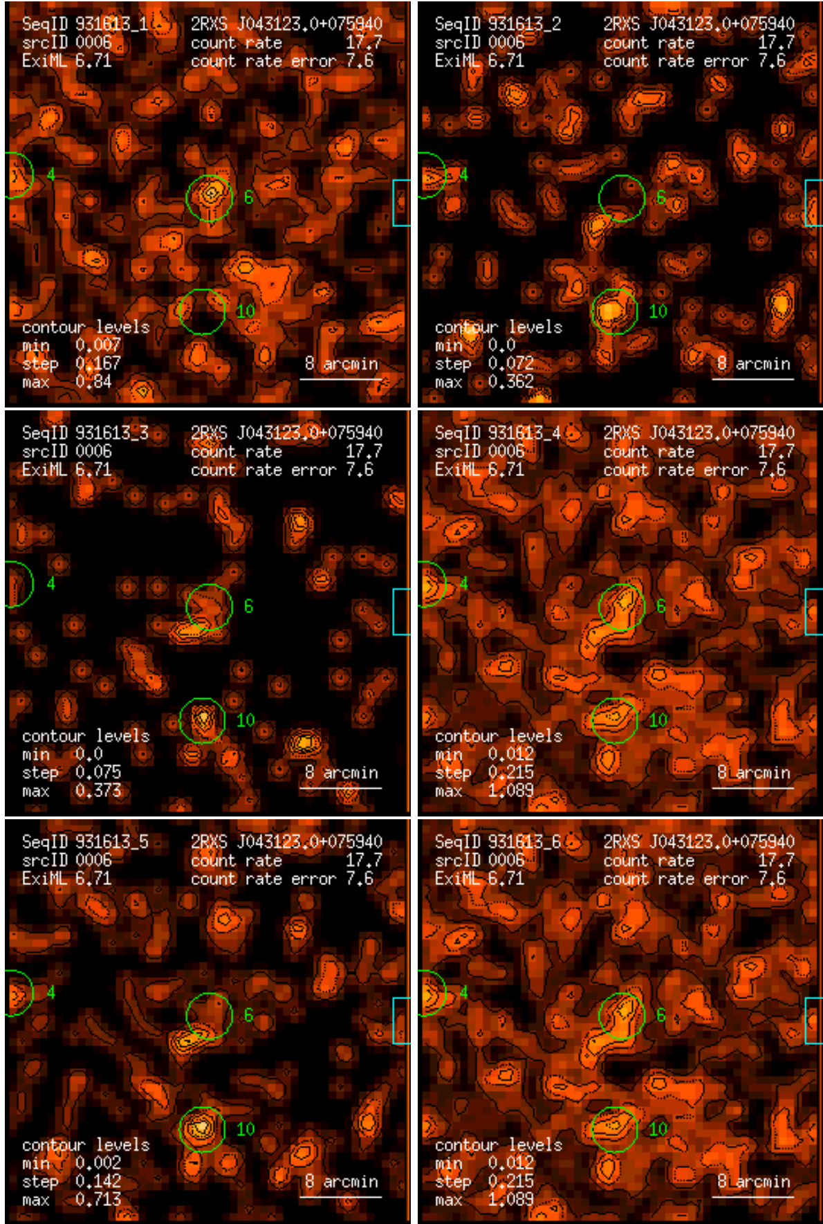
Figure 6: RASS 931613: detection 0006: band rate images, Gaussian filter: (1) PSPC channels 11 – 41, (2) 52 – 90, (3) 91 – 201, (4) 11 – 235, (5) 52 – 201, (6) 11 – 201. Broad band rates in counts/ks. Band rate contour levels in counts/ks/arcmin 2 .
