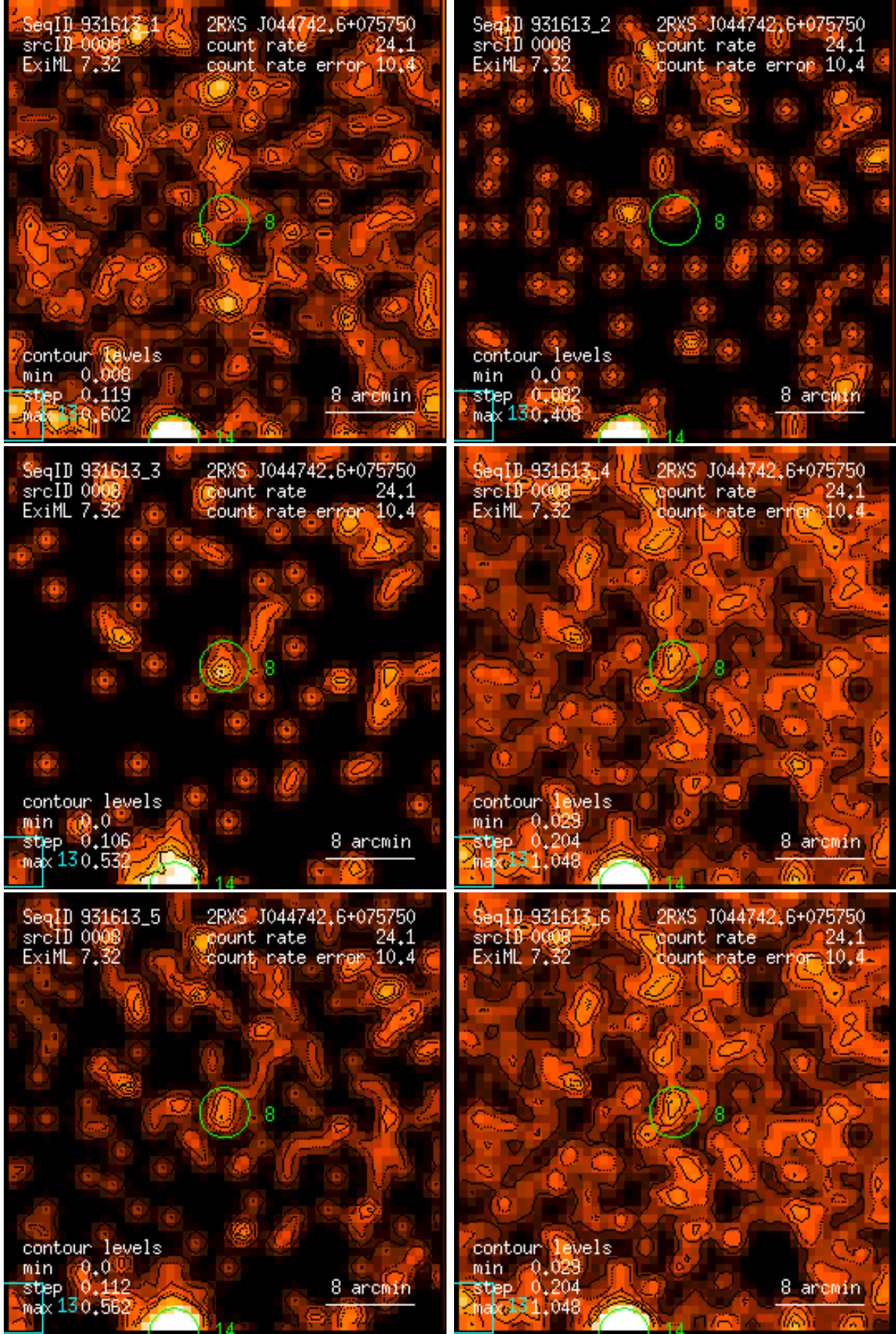
Figure 8: RASS 931613: detection 0008: band rate images, Gaussian filter: (1) PSPC channels 11 – 41, (2) 52 – 90, (3) 91 – 201, (4) 11 – 235, (5) 52 – 201, (6) 11 – 201. Broad band rates in counts/ks. Band rate contour levels in counts/ks/arcmin 2 .
