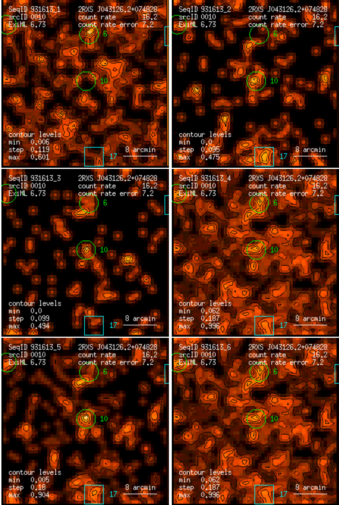
Figure 10: RASS 931613: detection 0010: band rate images, Gaussian filter: (1) PSPC channels 11 – 41, (2) 52 – 90, (3) 91 – 201, (4) 11 – 235, (5) 52 – 201, (6) 11 – 201. Broad band rates in counts/ks. Band rate contour levels in counts/ks/arcmin 2 .
