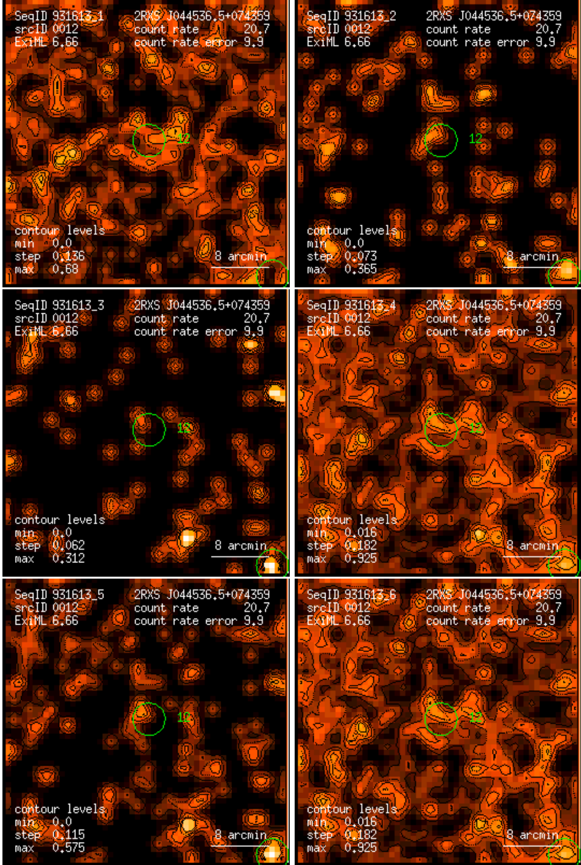
Figure 12: RASS 931613: detection 0012: band rate images, Gaussian filter: (1) PSPC channels 11 – 41, (2) 52 – 90, (3) 91 – 201, (4) 11 – 235, (5) 52 – 201, (6) 11 – 201. Broad band rates in counts/ks. Band rate contour levels in counts/ks/arcmin 2 .
