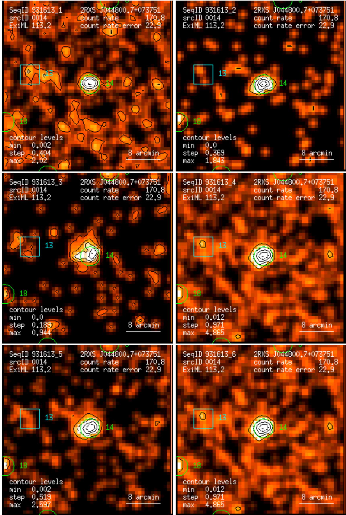
Figure 14: RASS 931613: detection 0014: band rate images, Gaussian filter: (1) PSPC channels 11 – 41, (2) 52 – 90, (3) 91 – 201, (4) 11 – 235, (5) 52 – 201, (6) 11 – 201. Broad band rates in counts/ks. Band rate contour levels in counts/ks/arcmin 2 .
