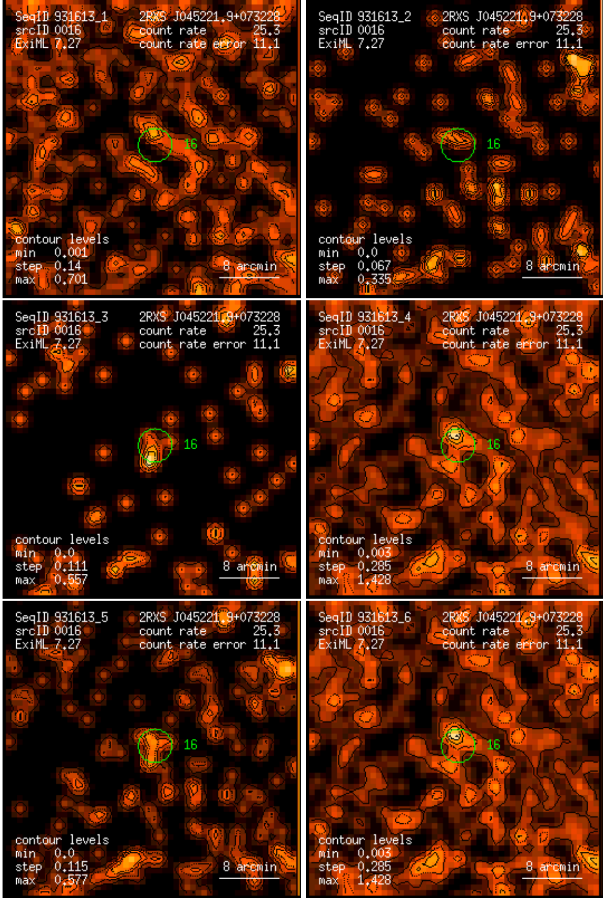
Figure 16: RASS 931613: detection 0016: band rate images, Gaussian filter: (1) PSPC channels 11 – 41, (2) 52 – 90, (3) 91 – 201, (4) 11 – 235, (5) 52 – 201, (6) 11 – 201. Broad band rates in counts/ks. Band rate contour levels in counts/ks/arcmin 2 .
