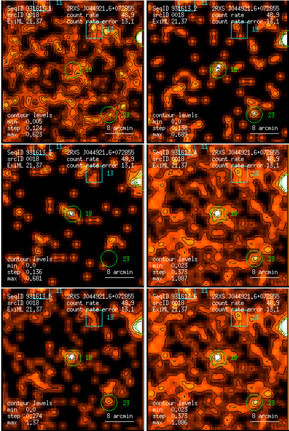
Figure 18: RASS 931613: detection 0018: band rate images, Gaussian filter: (1) PSPC channels 11 – 41, (2) 52 – 90, (3) 91 – 201, (4) 11 – 235, (5) 52 – 201, (6) 11 – 201. Broad band rates in counts/ks. Band rate contour levels in counts/ks/arcmin 2 .
