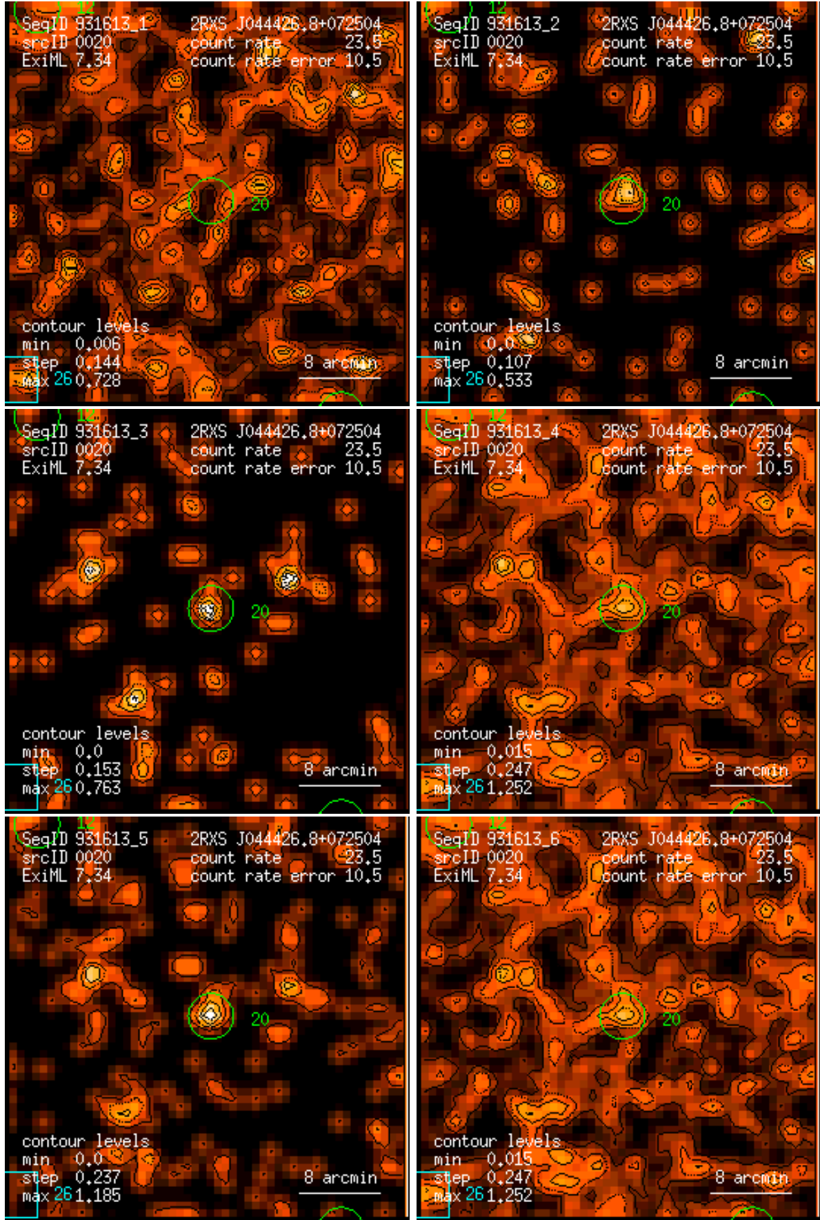
Figure 20: RASS 931613: detection 0020: band rate images, Gaussian filter: (1) PSPC channels 11 – 41, (2) 52 – 90, (3) 91 – 201, (4) 11 – 235, (5) 52 – 201, (6) 11 – 201. Broad band rates in counts/ks. Band rate contour levels in counts/ks/arcmin 2 .
