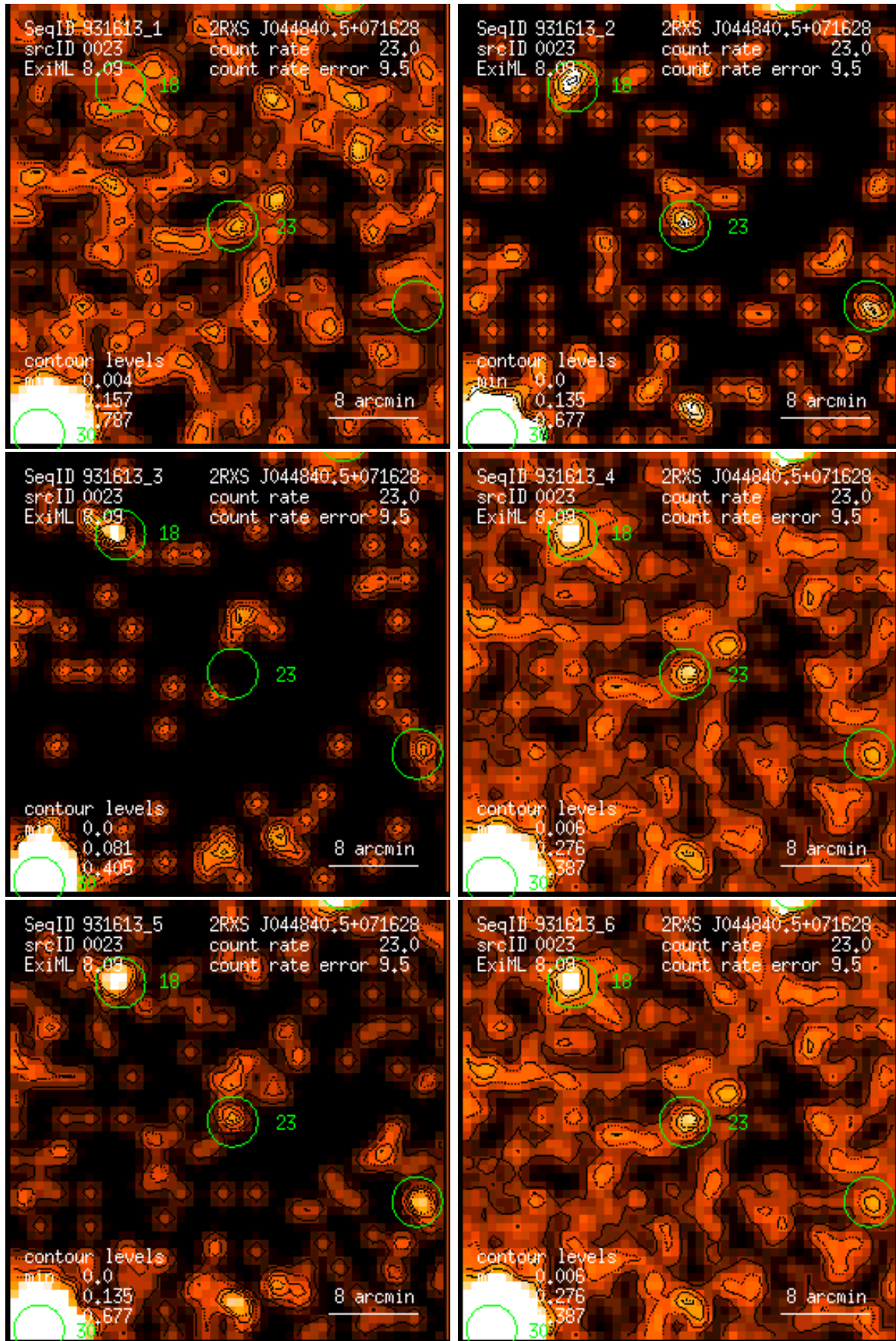
Figure 23: RASS 931613: detection 0023: band rate images, Gaussian filter: (1) PSPC channels 11 – 41, (2) 52 – 90, (3) 91 – 201, (4) 11 – 235, (5) 52 – 201, (6) 11 – 201. Broad band rates in counts/ks. Band rate contour levels in counts/ks/arcmin 2 .
