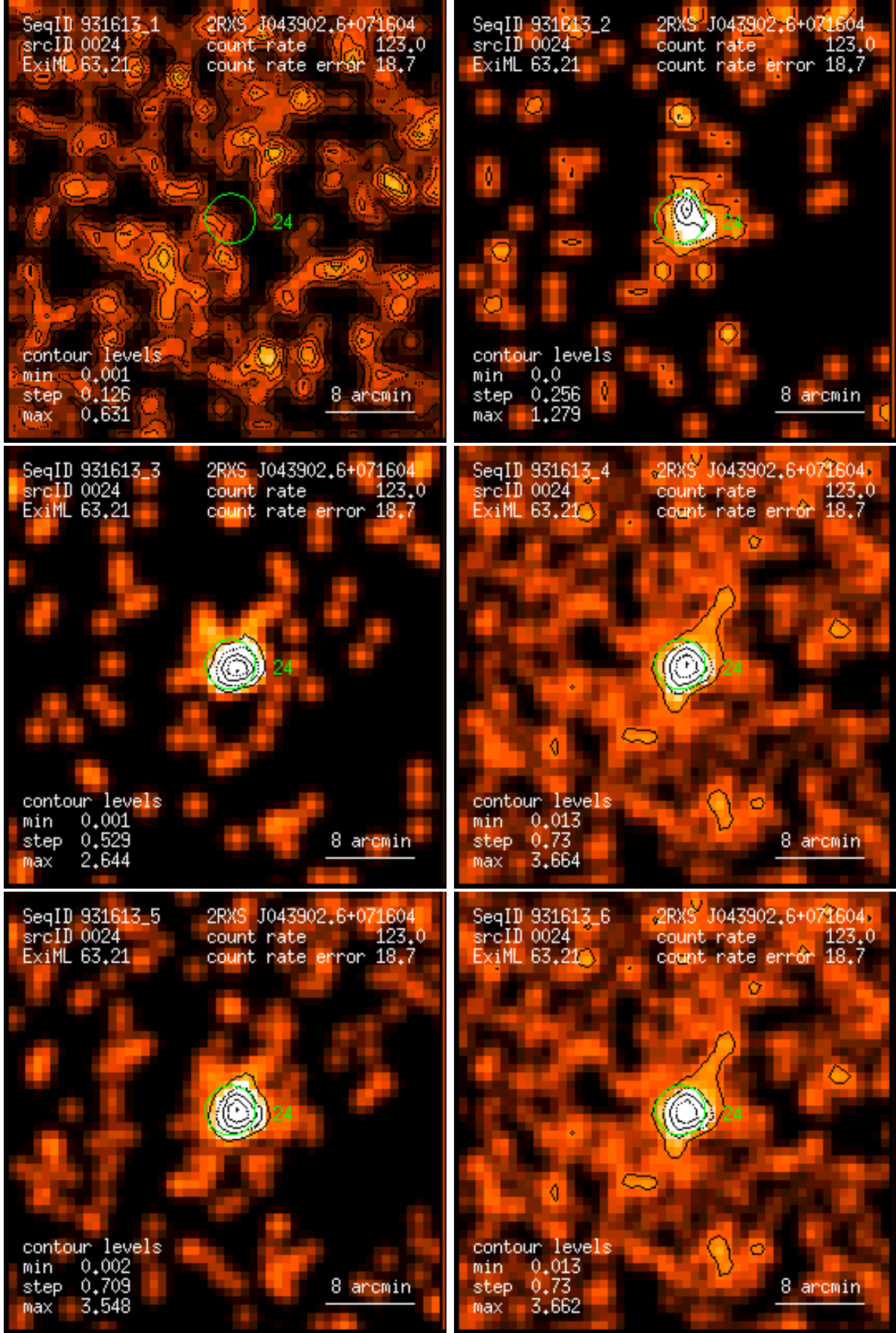
Figure 24: RASS 931613: detection 0024: band rate images, Gaussian filter: (1) PSPC channels 11 – 41, (2) 52 – 90, (3) 91 – 201, (4) 11 – 235, (5) 52 – 201, (6) 11 – 201. Broad band rates in counts/ks. Band rate contour levels in counts/ks/arcmin 2 .
