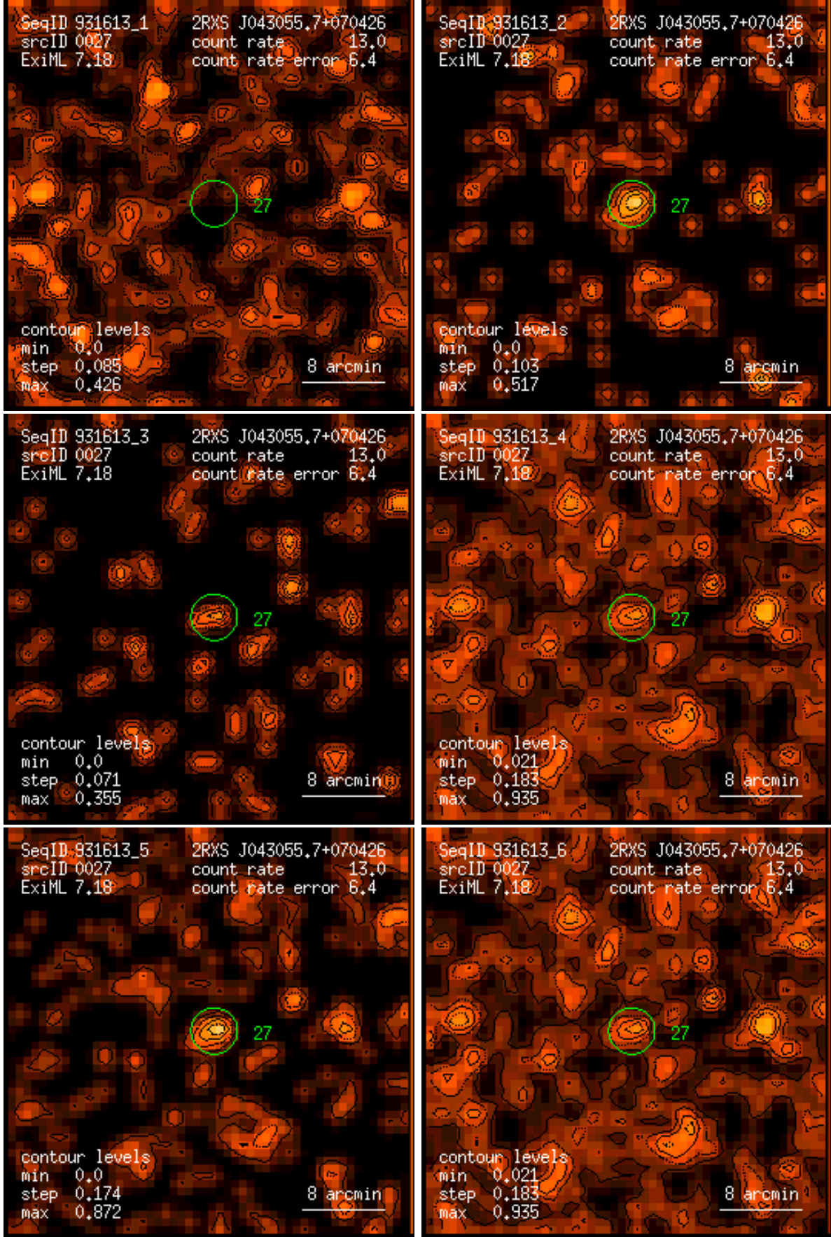
Figure 27: RASS 931613: detection 0027: band rate images, Gaussian filter: (1) PSPC channels 11 – 41, (2) 52 – 90, (3) 91 – 201, (4) 11 – 235, (5) 52 – 201, (6) 11 – 201. Broad band rates in counts/ks. Band rate contour levels in counts/ks/arcmin 2 .
