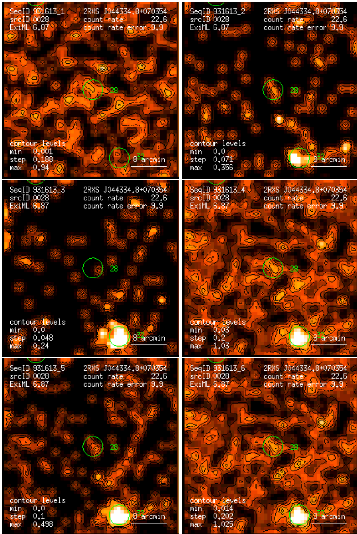
Figure 28: RASS 931613: detection 0028: band rate images, Gaussian filter: (1) PSPC channels 11 – 41, (2) 52 – 90, (3) 91 – 201, (4) 11 – 235, (5) 52 – 201, (6) 11 – 201. Broad band rates in counts/ks. Band rate contour levels in counts/ks/arcmin 2 .
