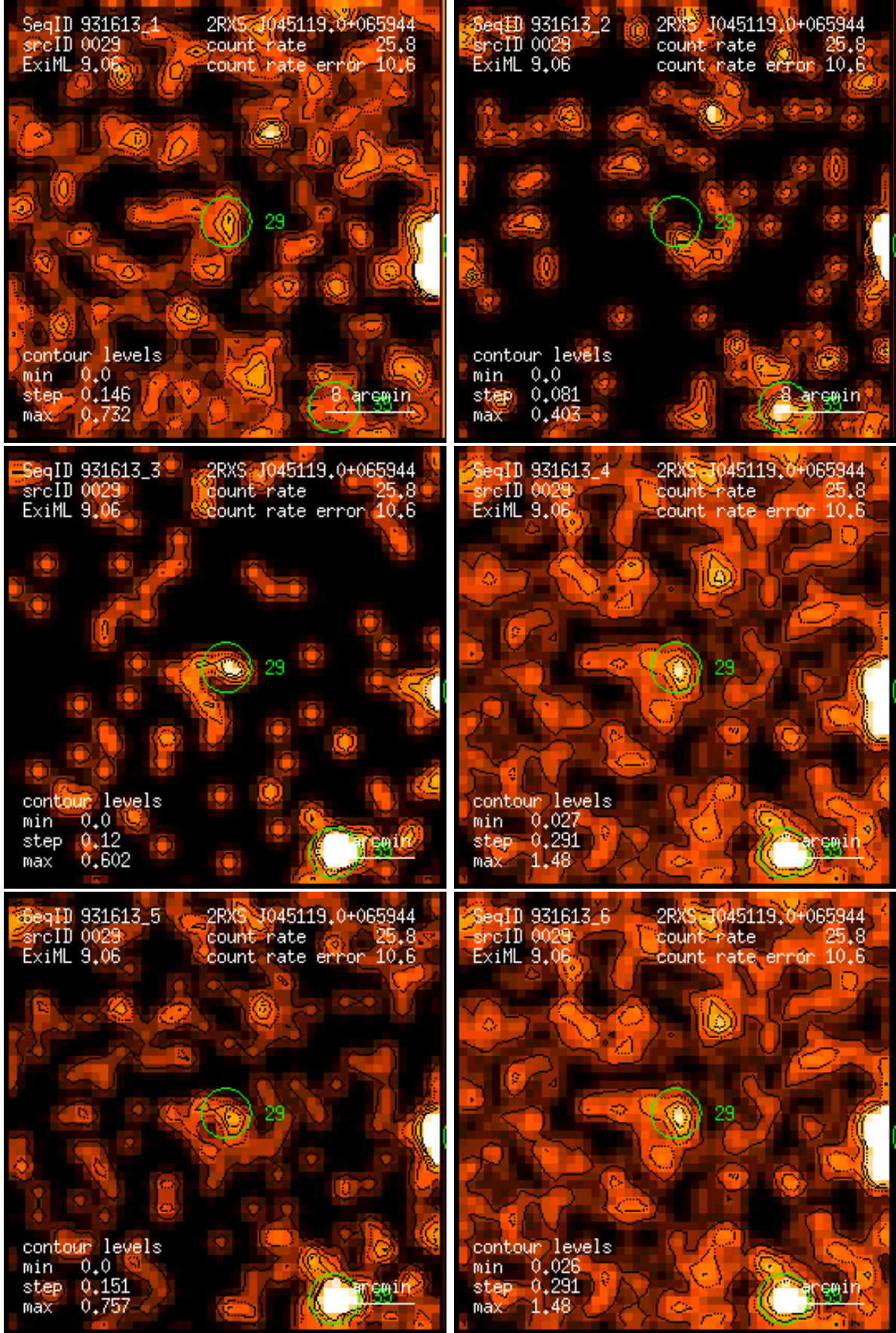
Figure 29: RASS 931613: detection 0029: band rate images, Gaussian filter: (1) PSPC channels 11 – 41, (2) 52 – 90, (3) 91 – 201, (4) 11 – 235, (5) 52 – 201, (6) 11 – 201. Broad band rates in counts/ks. Band rate contour levels in counts/ks/arcmin 2 .
