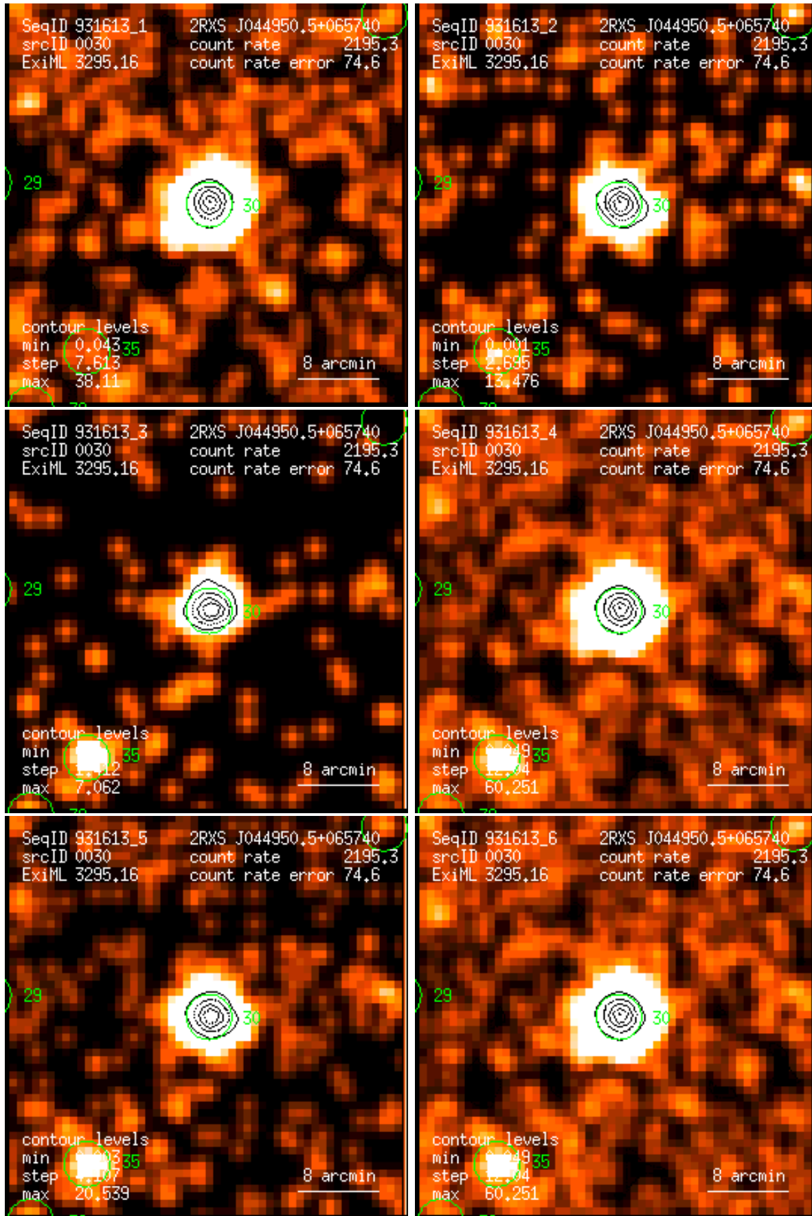
Figure 30: RASS 931613: detection 0030: band rate images, Gaussian filter: (1) PSPC channels 11 – 41, (2) 52 – 90, (3) 91 – 201, (4) 11 – 235, (5) 52 – 201, (6) 11 – 201. Broad band rates in counts/ks. Band rate contour levels in counts/ks/arcmin 2 .
