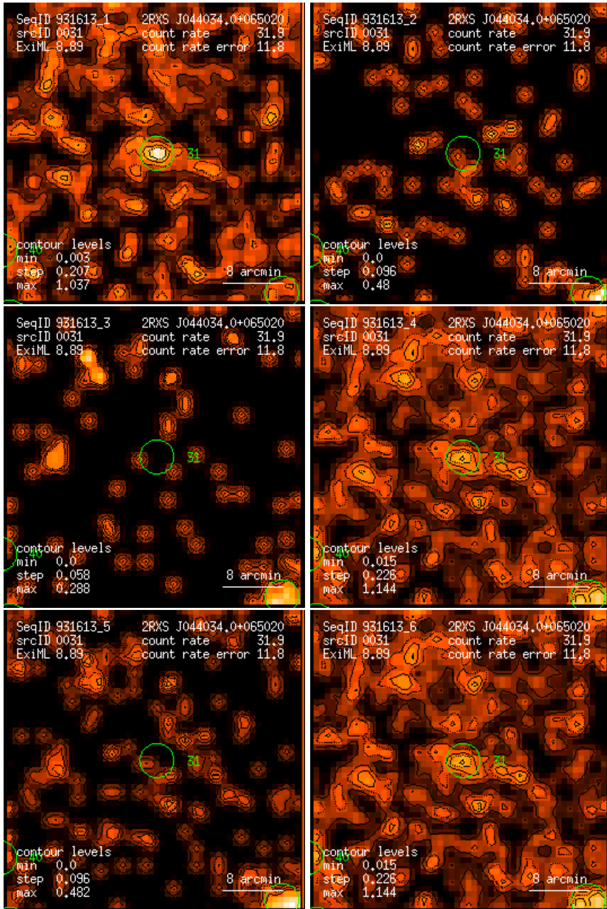
Figure 31: RASS 931613: detection 0031: band rate images, Gaussian filter: (1) PSPC channels 11 – 41, (2) 52 – 90, (3) 91 – 201, (4) 11 – 235, (5) 52 – 201, (6) 11 – 201. Broad band rates in counts/ks. Band rate contour levels in counts/ks/arcmin 2 .
