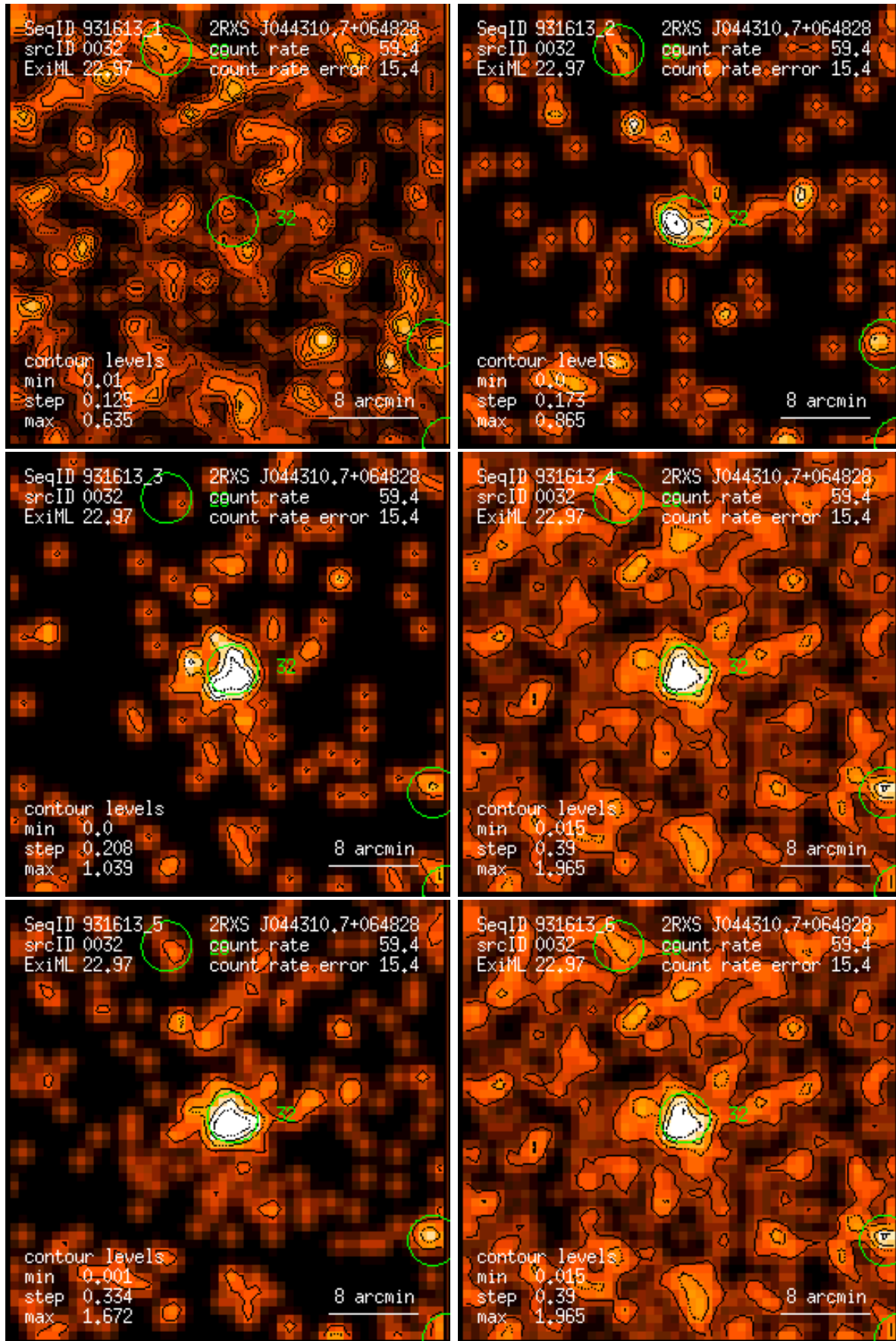
Figure 32: RASS 931613: detection 0032: band rate images, Gaussian filter: (1) PSPC channels 11 – 41, (2) 52 – 90, (3) 91 – 201, (4) 11 – 235, (5) 52 – 201, (6) 11 – 201. Broad band rates in counts/ks. Band rate contour levels in counts/ks/arcmin 2 .
