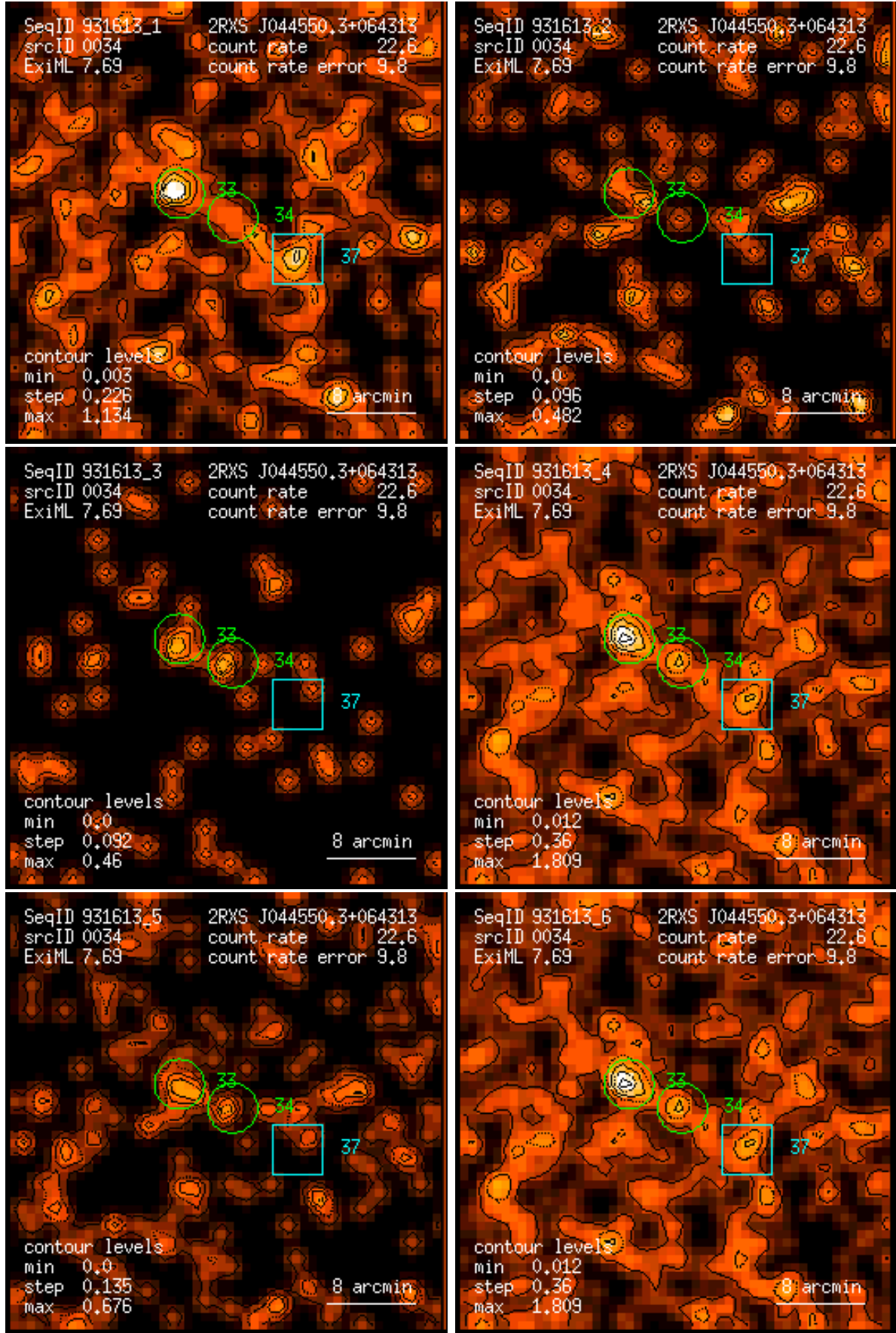
Figure 34: RASS 931613: detection 0034: band rate images, Gaussian filter: (1) PSPC channels 11 – 41, (2) 52 – 90, (3) 91 – 201, (4) 11 – 235, (5) 52 – 201, (6) 11 – 201. Broad band rates in counts/ks. Band rate contour levels in counts/ks/arcmin 2 .
