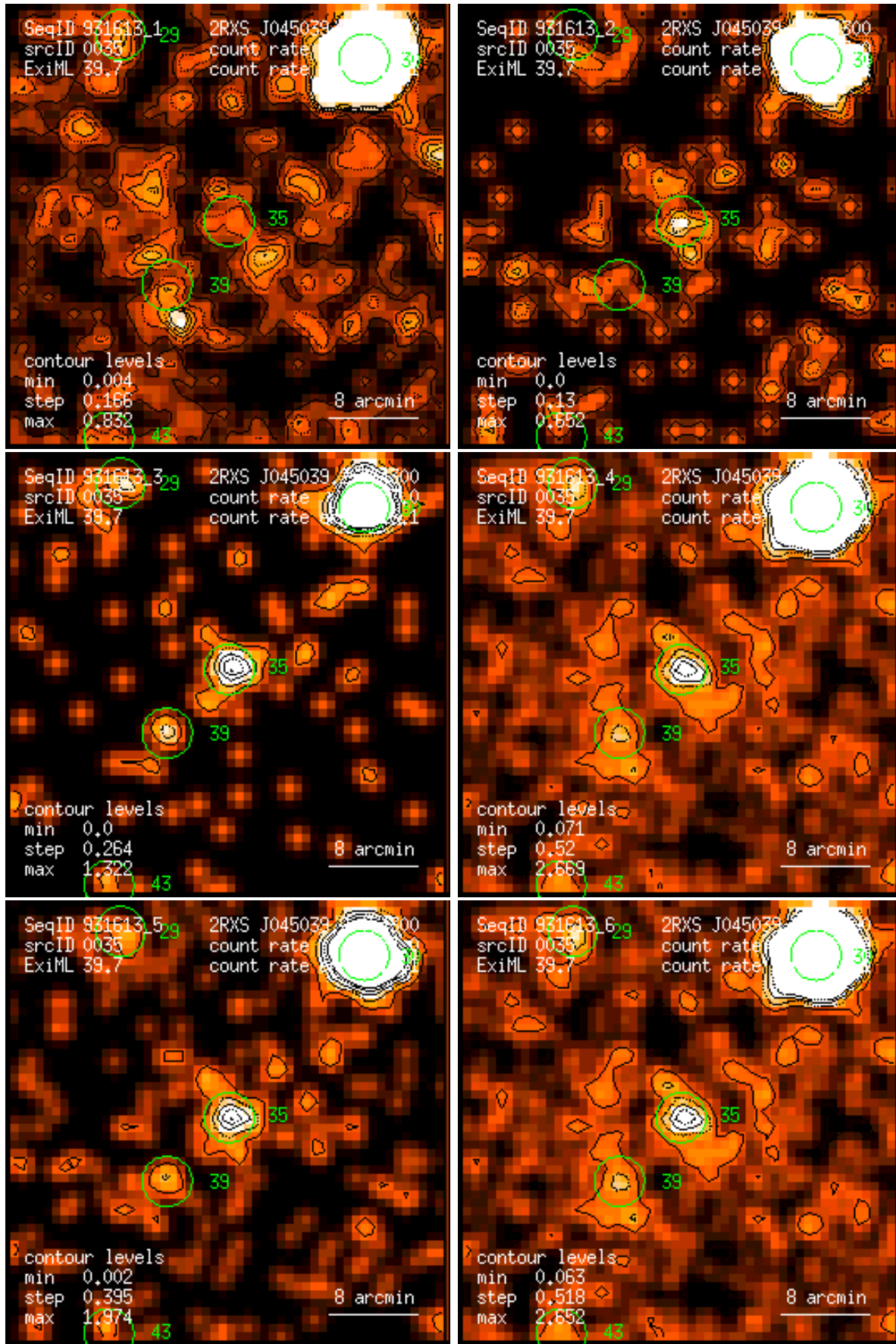
Figure 35: RASS 931613: detection 0035: band rate images, Gaussian filter: (1) PSPC channels 11 – 41, (2) 52 – 90, (3) 91 – 201, (4) 11 – 235, (5) 52 – 201, (6) 11 – 201. Broad band rates in counts/ks. Band rate contour levels in counts/ks/arcmin 2 .
