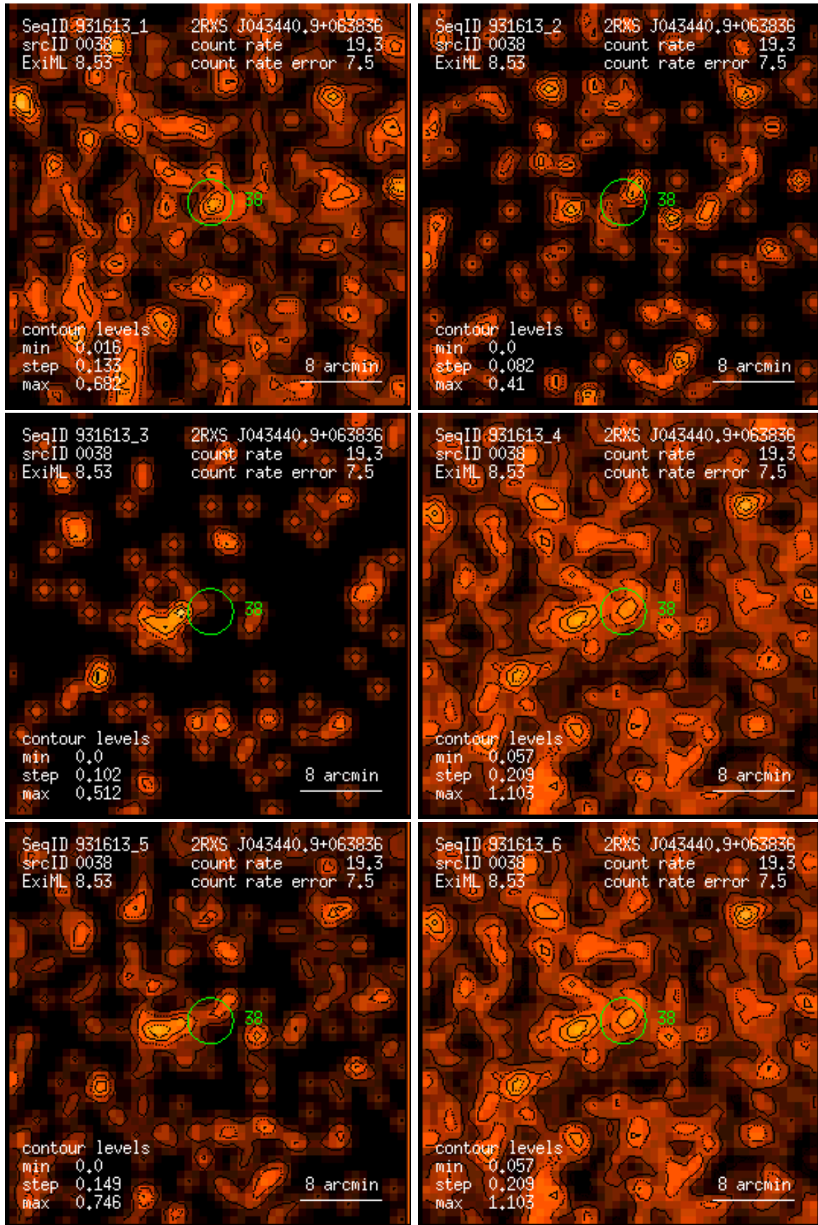
Figure 38: RASS 931613: detection 0038: band rate images, Gaussian filter: (1) PSPC channels 11 – 41, (2) 52 – 90, (3) 91 – 201, (4) 11 – 235, (5) 52 – 201, (6) 11 – 201. Broad band rates in counts/ks. Band rate contour levels in counts/ks/arcmin 2 .
