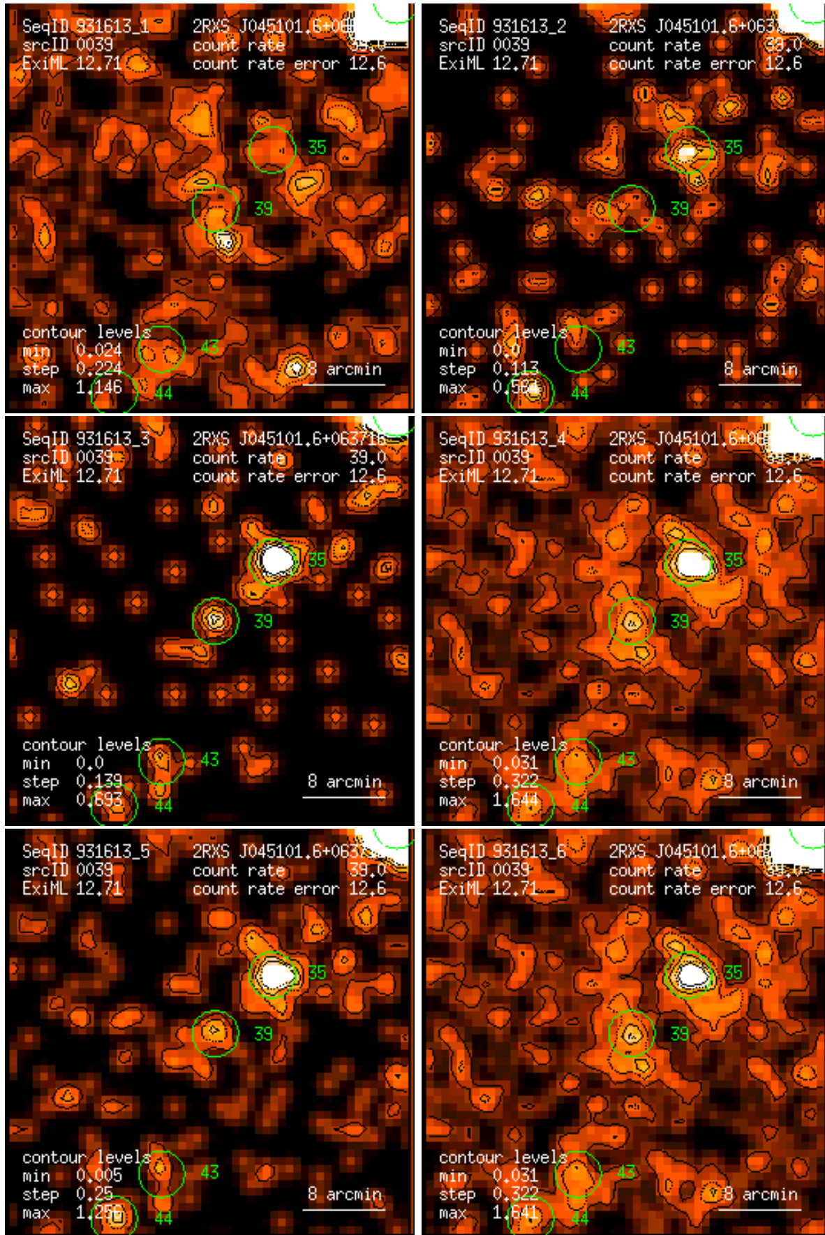
Figure 39: RASS 931613: detection 0039: band rate images, Gaussian filter: (1) PSPC channels 11 – 41, (2) 52 – 90, (3) 91 – 201, (4) 11 – 235, (5) 52 – 201, (6) 11 – 201. Broad band rates in counts/ks. Band rate contour levels in counts/ks/arcmin 2 .
