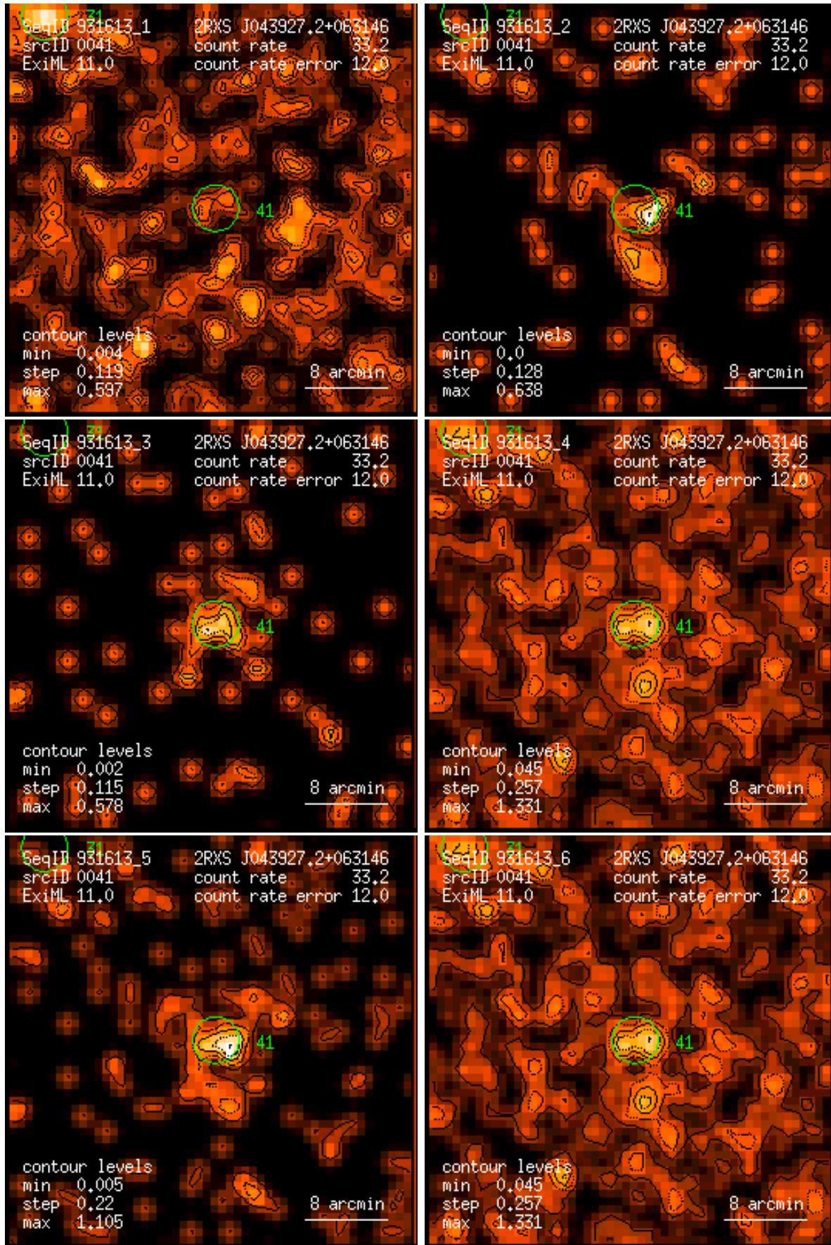
Figure 41: RASS 931613: detection 0041: band rate images, Gaussian filter: (1) PSPC channels 11 – 41, (2) 52 – 90, (3) 91 – 201, (4) 11 – 235, (5) 52 – 201, (6) 11 – 201. Broad band rates in counts/ks. Band rate contour levels in counts/ks/arcmin 2 .
