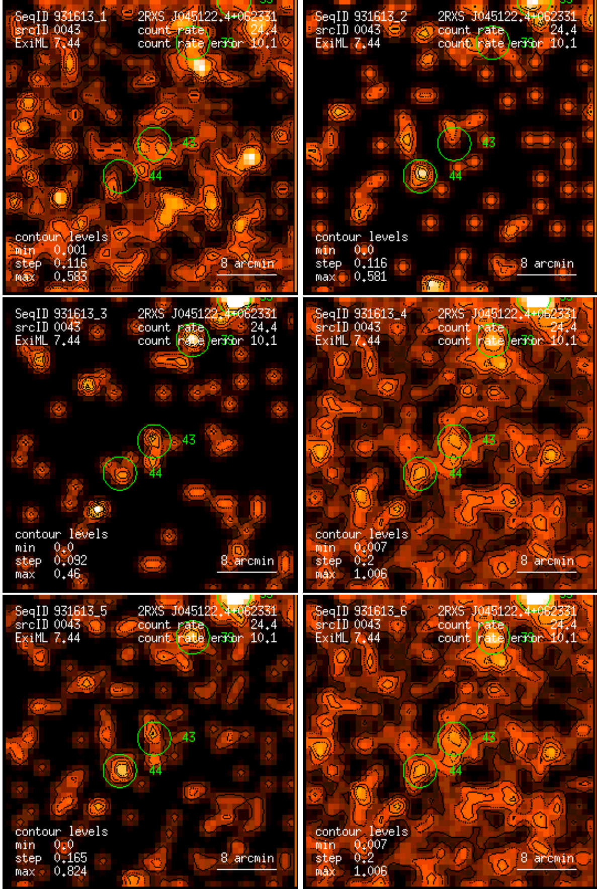
Figure 43: RASS 931613: detection 0043: band rate images, Gaussian filter: (1) PSPC channels 11 – 41, (2) 52 – 90, (3) 91 – 201, (4) 11 – 235, (5) 52 – 201, (6) 11 – 201. Broad band rates in counts/ks. Band rate contour levels in counts/ks/arcmin 2 .
