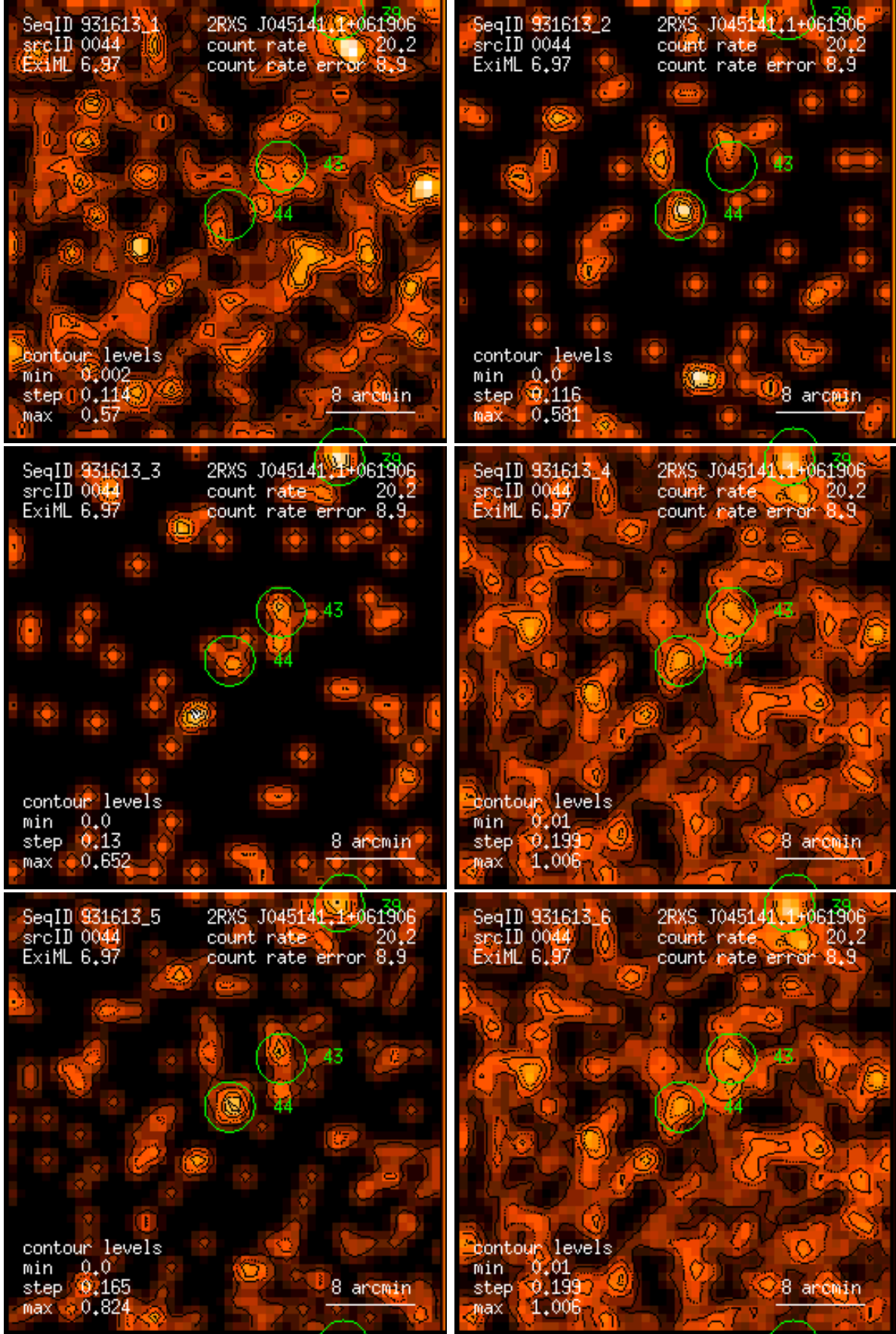
Figure 44: RASS 931613: detection 0044: band rate images, Gaussian filter: (1) PSPC channels 11 – 41, (2) 52 – 90, (3) 91 – 201, (4) 11 – 235, (5) 52 – 201, (6) 11 – 201. Broad band rates in counts/ks. Band rate contour levels in counts/ks/arcmin 2 .
