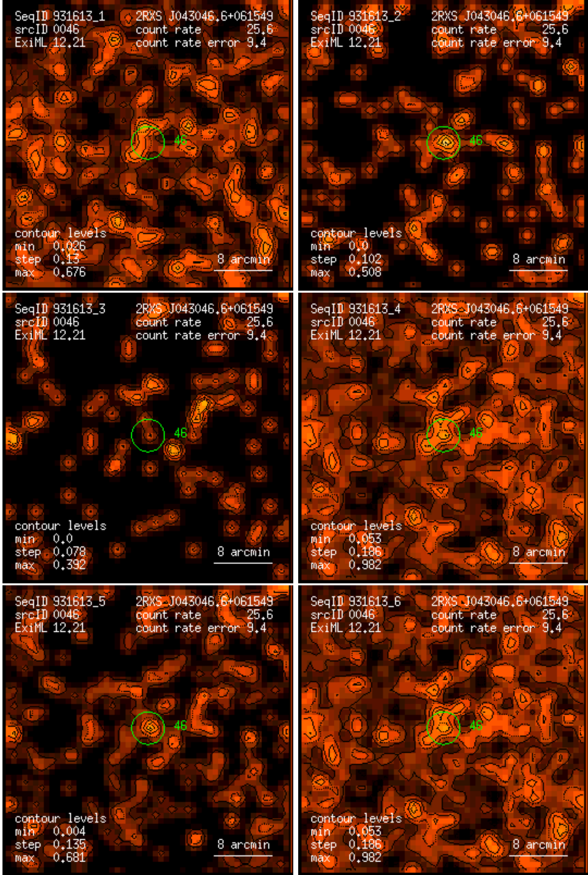
Figure 46: RASS 931613: detection 0046: band rate images, Gaussian filter: (1) PSPC channels 11 – 41, (2) 52 – 90, (3) 91 – 201, (4) 11 – 235, (5) 52 – 201, (6) 11 – 201. Broad band rates in counts/ks. Band rate contour levels in counts/ks/arcmin 2 .
