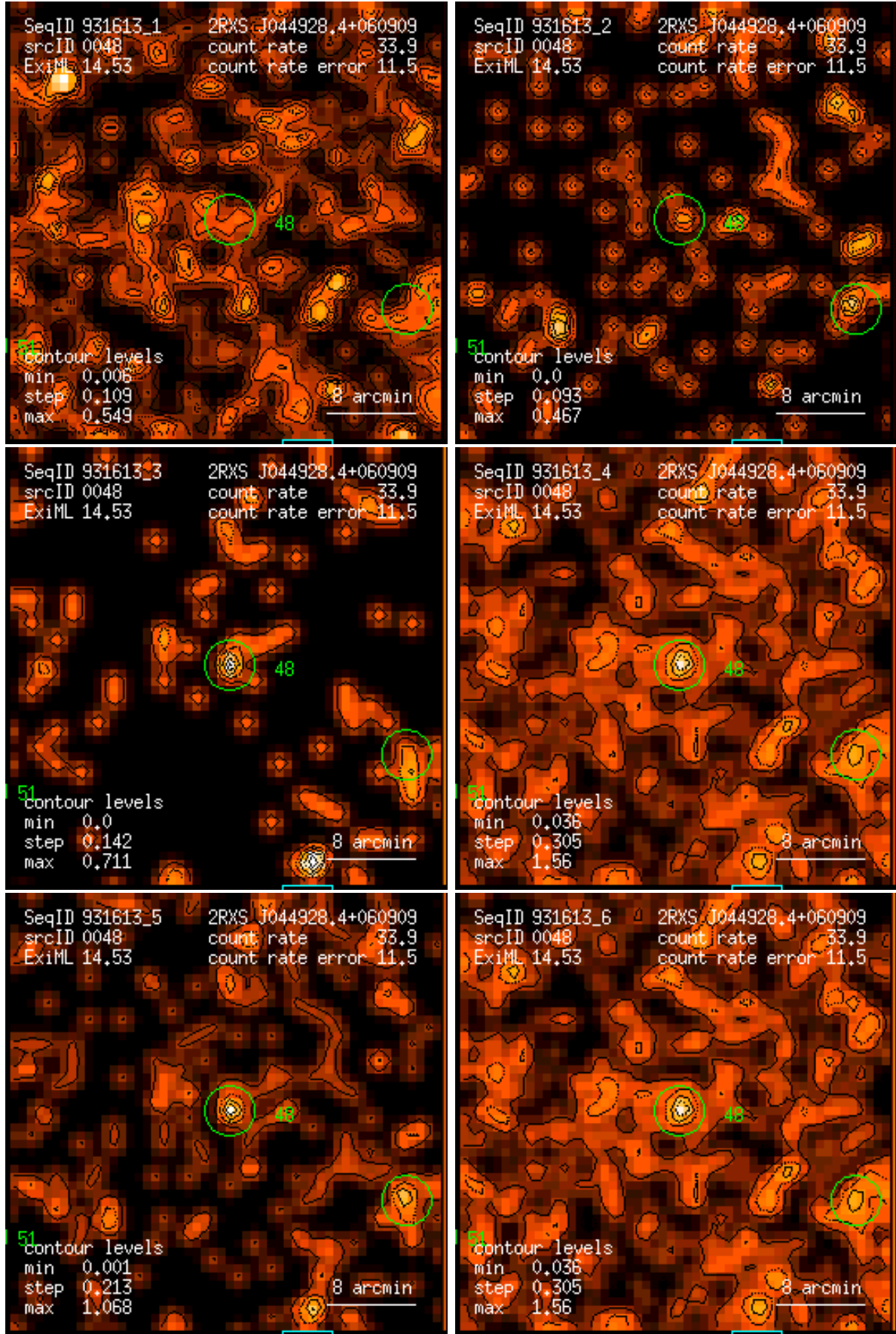
Figure 48: RASS 931613: detection 0048: band rate images, Gaussian filter: (1) PSPC channels 11 – 41, (2) 52 – 90, (3) 91 – 201, (4) 11 – 235, (5) 52 – 201, (6) 11 – 201. Broad band rates in counts/ks. Band rate contour levels in counts/ks/arcmin 2 .
