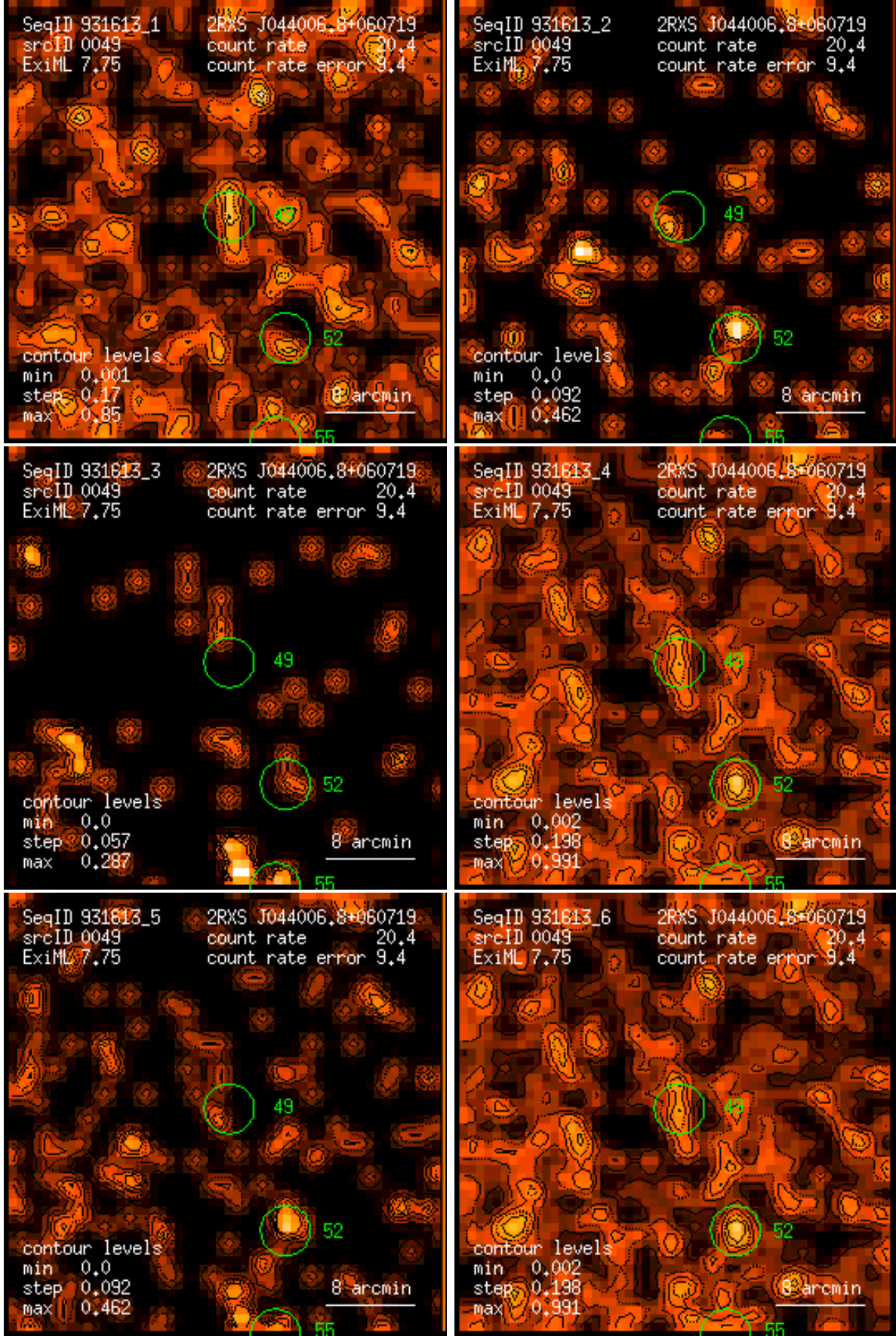
Figure 49: RASS 931613: detection 0049: band rate images, Gaussian filter: (1) PSPC channels 11 – 41, (2) 52 – 90, (3) 91 – 201, (4) 11 – 235, (5) 52 – 201, (6) 11 – 201. Broad band rates in counts/ks. Band rate contour levels in counts/ks/arcmin 2 .
