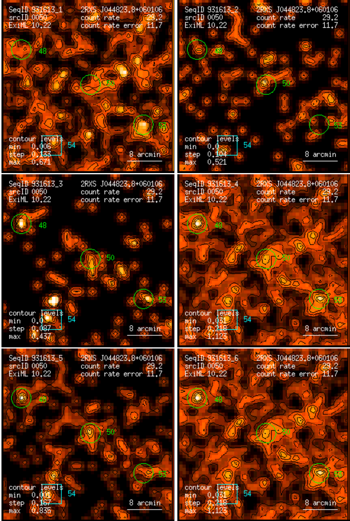
Figure 50: RASS 931613: detection 0050: band rate images, Gaussian filter: (1) PSPC channels 11 – 41, (2) 52 – 90, (3) 91 – 201, (4) 11 – 235, (5) 52 – 201, (6) 11 – 201. Broad band rates in counts/ks. Band rate contour levels in counts/ks/arcmin 2 .
