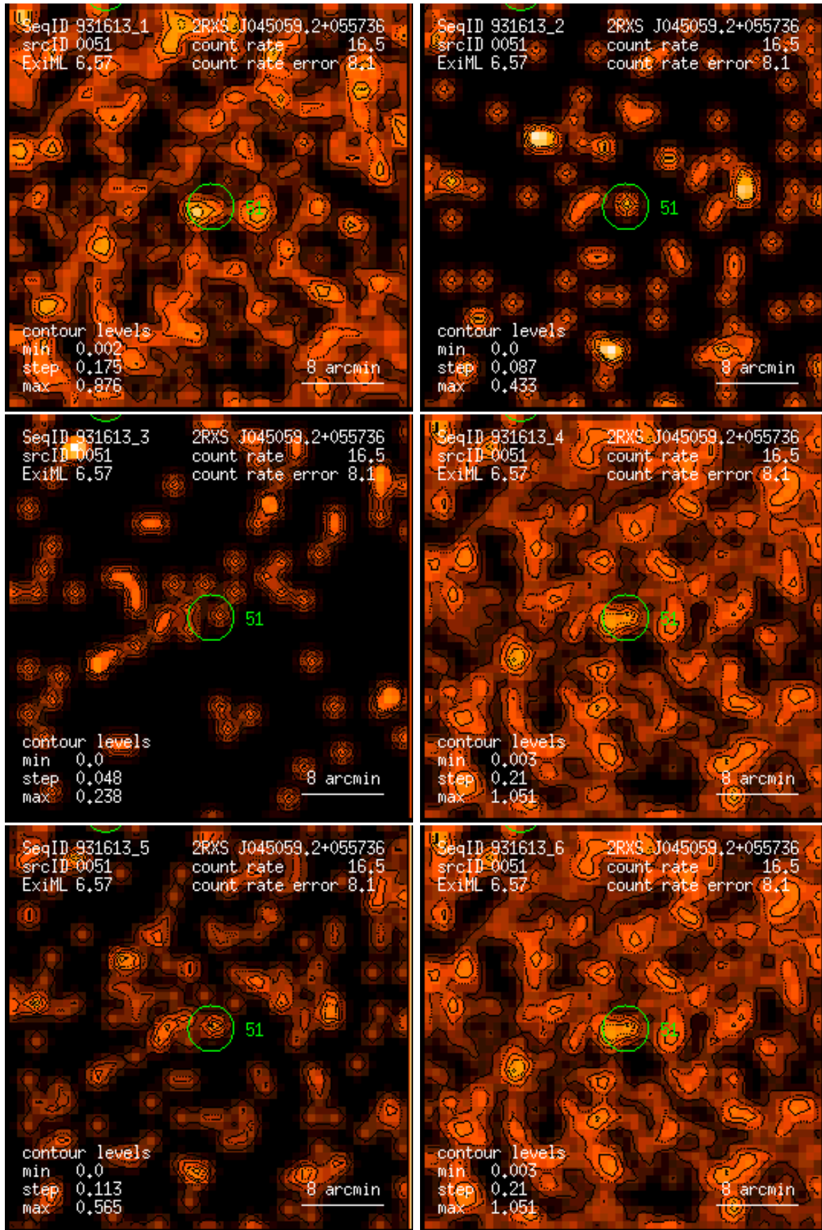
Figure 51: RASS 931613: detection 0051: band rate images, Gaussian filter: (1) PSPC channels 11 – 41, (2) 52 – 90, (3) 91 – 201, (4) 11 – 235, (5) 52 – 201, (6) 11 – 201. Broad band rates in counts/ks. Band rate contour levels in counts/ks/arcmin 2 .
