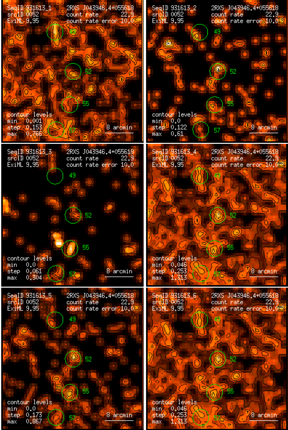
Figure 52: RASS 931613: detection 0052: band rate images, Gaussian filter: (1) PSPC channels 11 – 41, (2) 52 – 90, (3) 91 – 201, (4) 11 – 235, (5) 52 – 201, (6) 11 – 201. Broad band rates in counts/ks. Band rate contour levels in counts/ks/arcmin 2 .
