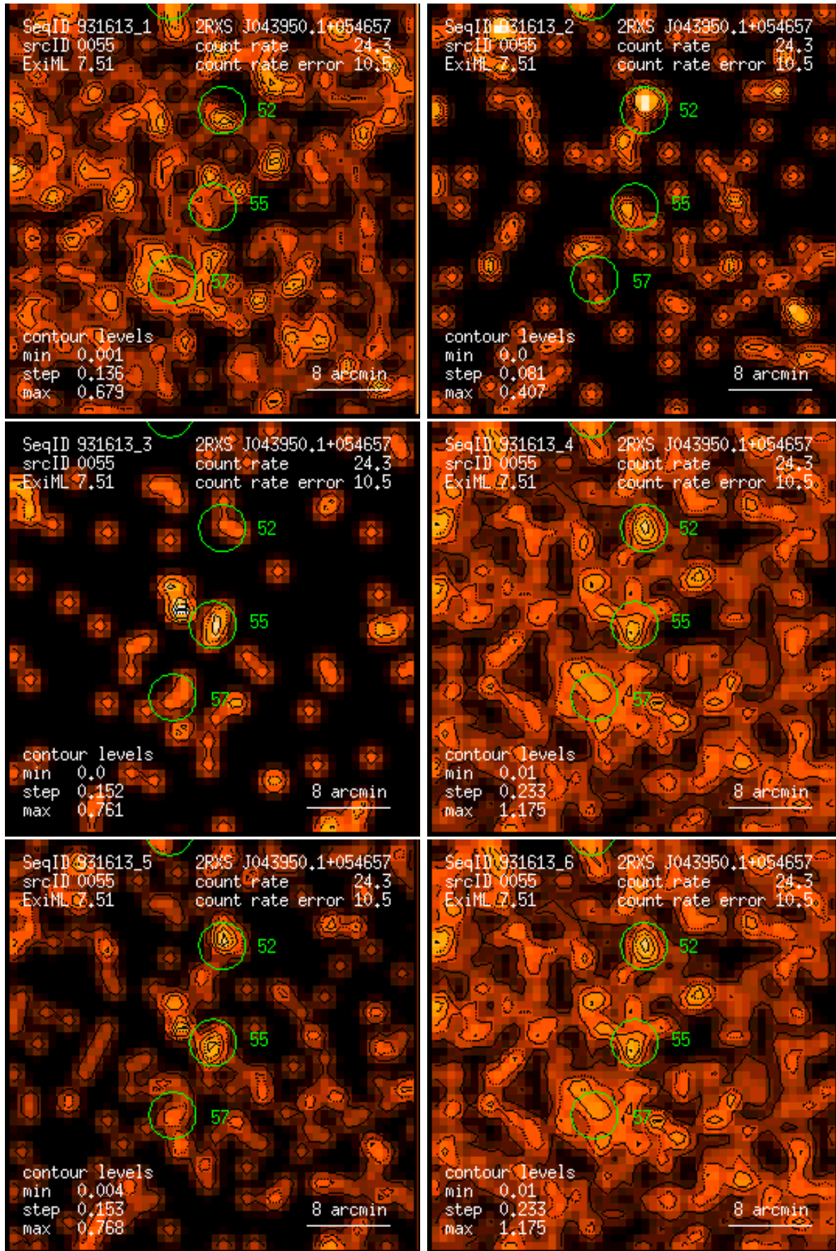
Figure 55: RASS 931613: detection 0055: band rate images, Gaussian filter: (1) PSPC channels 11 – 41, (2) 52 – 90, (3) 91 – 201, (4) 11 – 235, (5) 52 – 201, (6) 11 – 201. Broad band rates in counts/ks. Band rate contour levels in counts/ks/arcmin 2 .
