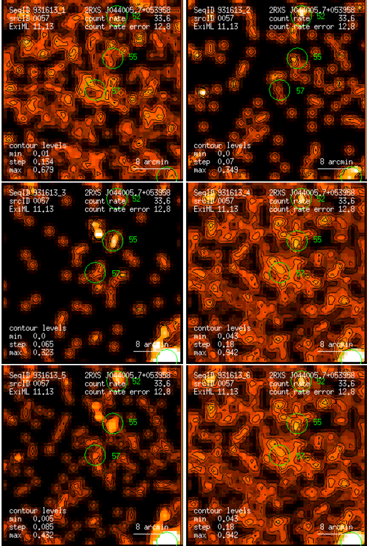
Figure 57: RASS 931613: detection 0057: band rate images, Gaussian filter: (1) PSPC channels 11 – 41, (2) 52 – 90, (3) 91 – 201, (4) 11 – 235, (5) 52 – 201, (6) 11 – 201. Broad band rates in counts/ks. Band rate contour levels in counts/ks/arcmin 2 .
