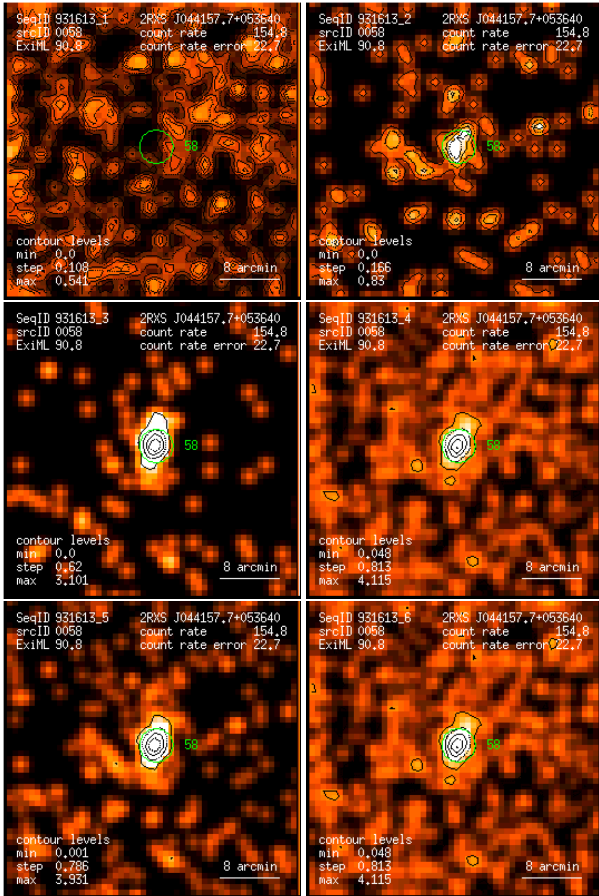
Figure 58: RASS 931613: detection 0058: band rate images, Gaussian filter: (1) PSPC channels 11 – 41, (2) 52 – 90, (3) 91 – 201, (4) 11 – 235, (5) 52 – 201, (6) 11 – 201. Broad band rates in counts/ks. Band rate contour levels in counts/ks/arcmin 2 .
