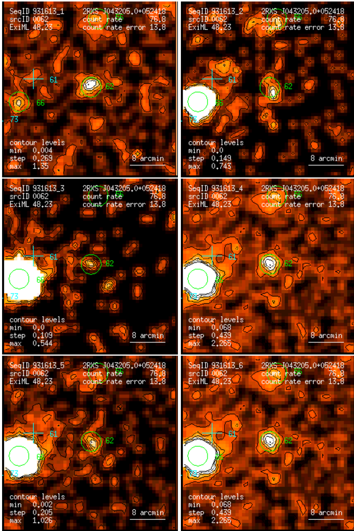
Figure 62: RASS 931613: detection 0062: band rate images, Gaussian filter: (1) PSPC channels 11 – 41, (2) 52 – 90, (3) 91 – 201, (4) 11 – 235, (5) 52 – 201, (6) 11 – 201. Broad band rates in counts/ks. Band rate contour levels in counts/ks/arcmin 2 .
