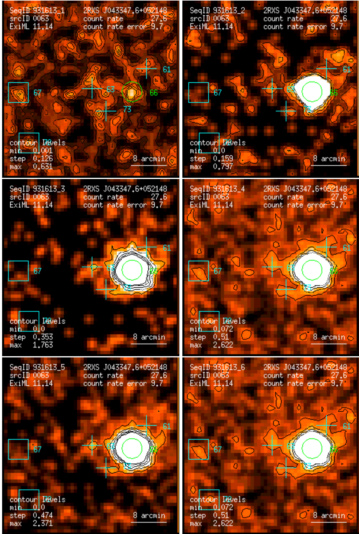
Figure 63: RASS 931613: detection 0063: band rate images, Gaussian filter: (1) PSPC channels 11 – 41, (2) 52 – 90, (3) 91 – 201, (4) 11 – 235, (5) 52 – 201, (6) 11 – 201. Broad band rates in counts/ks. Band rate contour levels in counts/ks/arcmin 2 .
