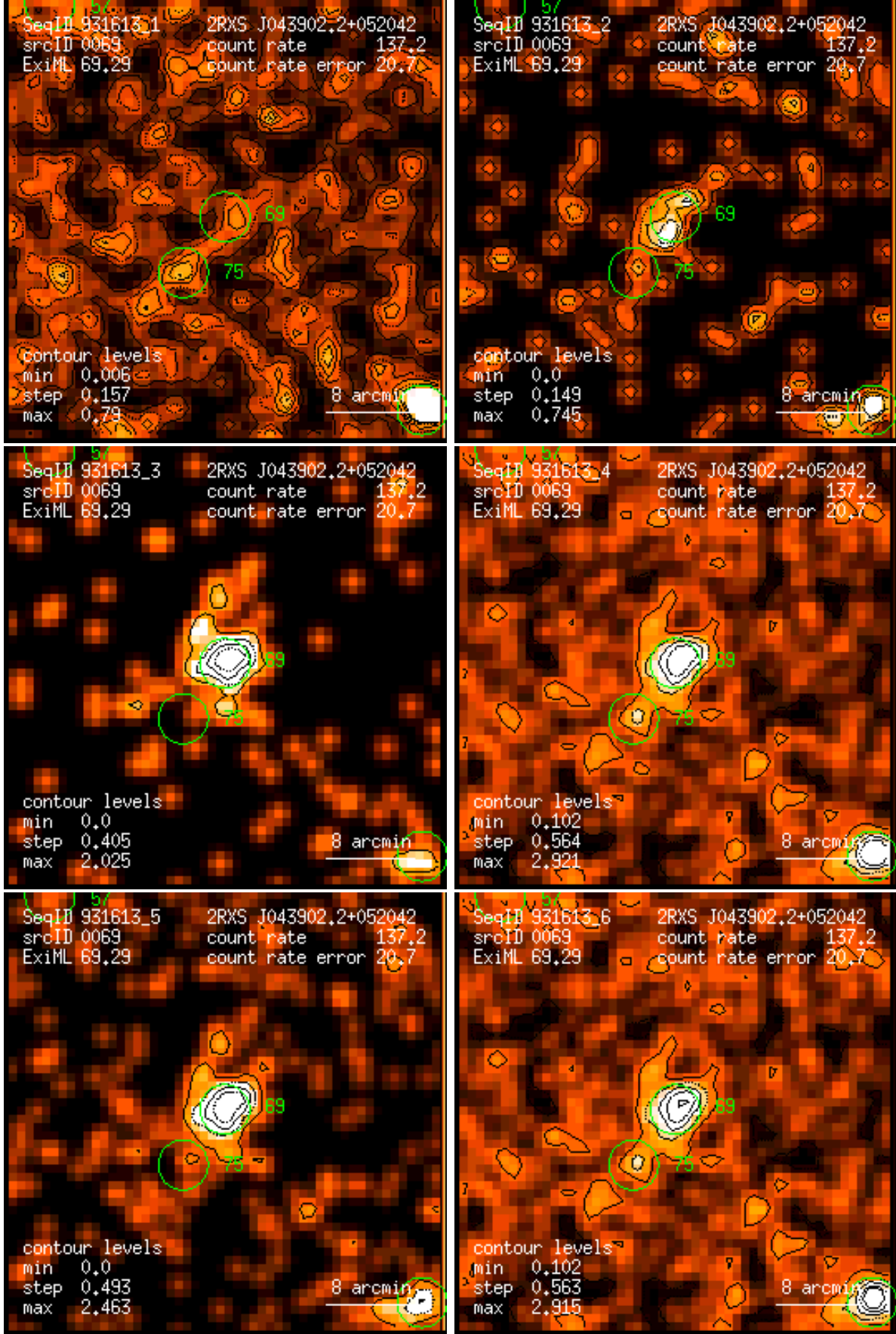
Figure 69: RASS 931613: detection 0069: band rate images, Gaussian filter: (1) PSPC channels 11 – 41, (2) 52 – 90, (3) 91 – 201, (4) 11 – 235, (5) 52 – 201, (6) 11 – 201. Broad band rates in counts/ks. Band rate contour levels in counts/ks/arcmin 2 .
