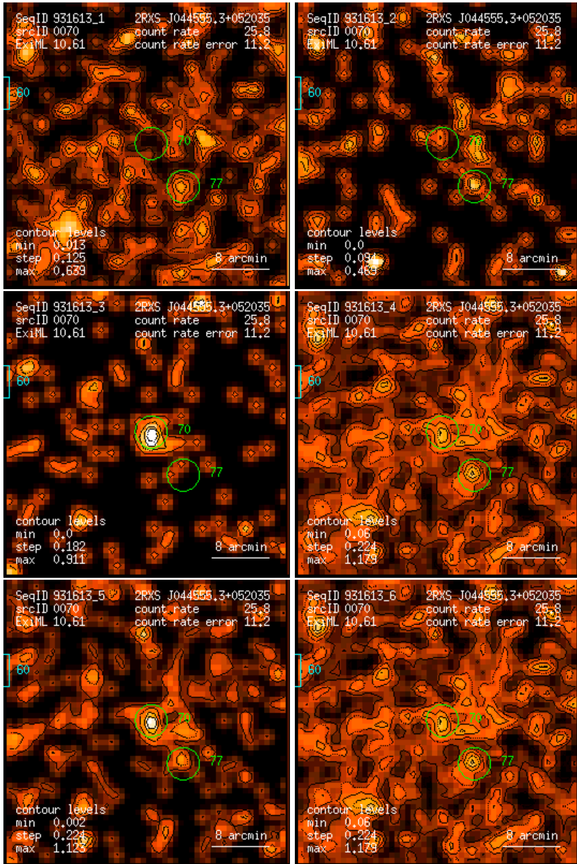
Figure 70: RASS 931613: detection 0070: band rate images, Gaussian filter: (1) PSPC channels 11 – 41, (2) 52 – 90, (3) 91 – 201, (4) 11 – 235, (5) 52 – 201, (6) 11 – 201. Broad band rates in counts/ks. Band rate contour levels in counts/ks/arcmin 2 .
