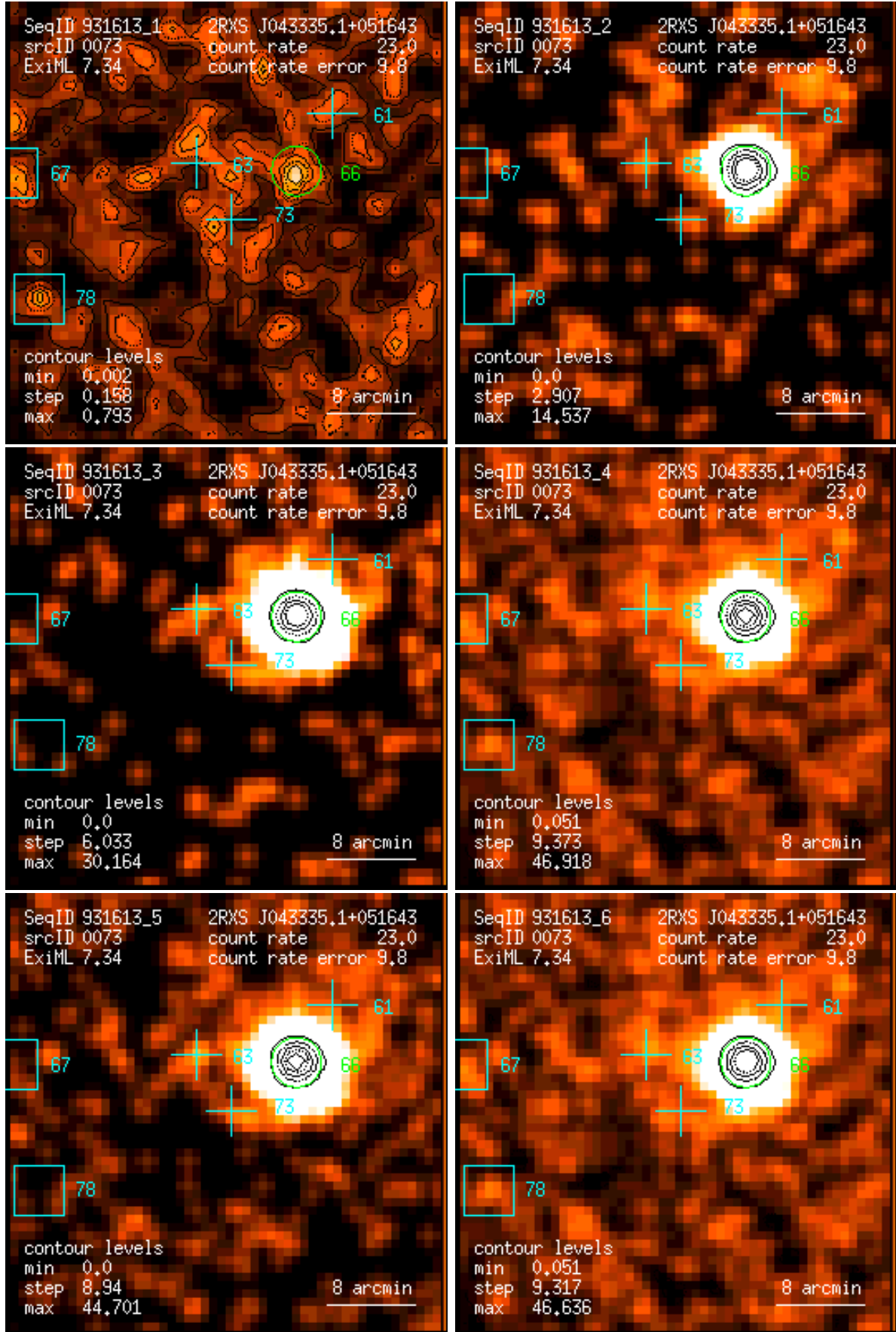
Figure 73: RASS 931613: detection 0073: band rate images, Gaussian filter: (1) PSPC channels 11 – 41, (2) 52 – 90, (3) 91 – 201, (4) 11 – 235, (5) 52 – 201, (6) 11 – 201. Broad band rates in counts/ks. Band rate contour levels in counts/ks/arcmin 2 .
