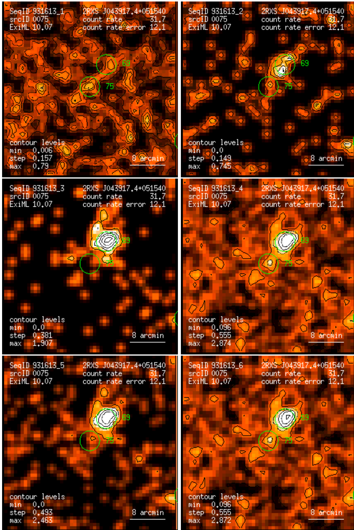
Figure 75: RASS 931613: detection 0075: band rate images, Gaussian filter: (1) PSPC channels 11 – 41, (2) 52 – 90, (3) 91 – 201, (4) 11 – 235, (5) 52 – 201, (6) 11 – 201. Broad band rates in counts/ks. Band rate contour levels in counts/ks/arcmin 2 .
