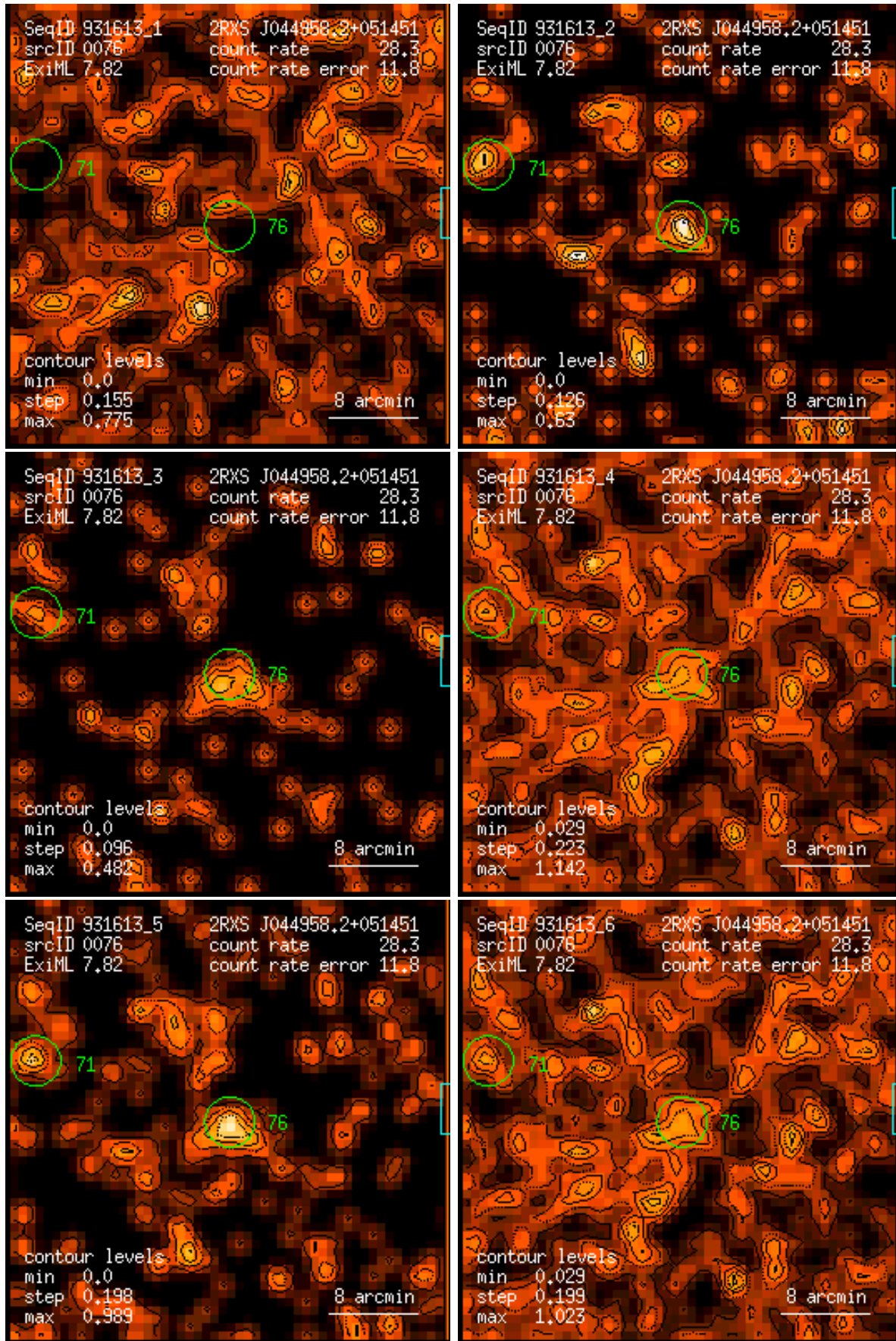
Figure 76: RASS 931613: detection 0076: band rate images, Gaussian filter: (1) PSPC channels 11 – 41, (2) 52 – 90, (3) 91 – 201, (4) 11 – 235, (5) 52 – 201, (6) 11 – 201. Broad band rates in counts/ks. Band rate contour levels in counts/ks/arcmin 2 .
