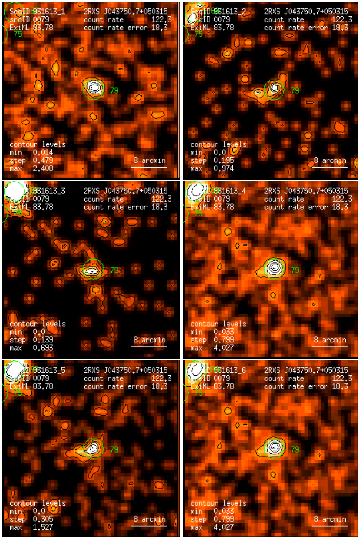
Figure 79: RASS 931613: detection 0079: band rate images, Gaussian filter: (1) PSPC channels 11 – 41, (2) 52 – 90, (3) 91 – 201, (4) 11 – 235, (5) 52 – 201, (6) 11 – 201. Broad band rates in counts/ks. Band rate contour levels in counts/ks/arcmin 2 .
