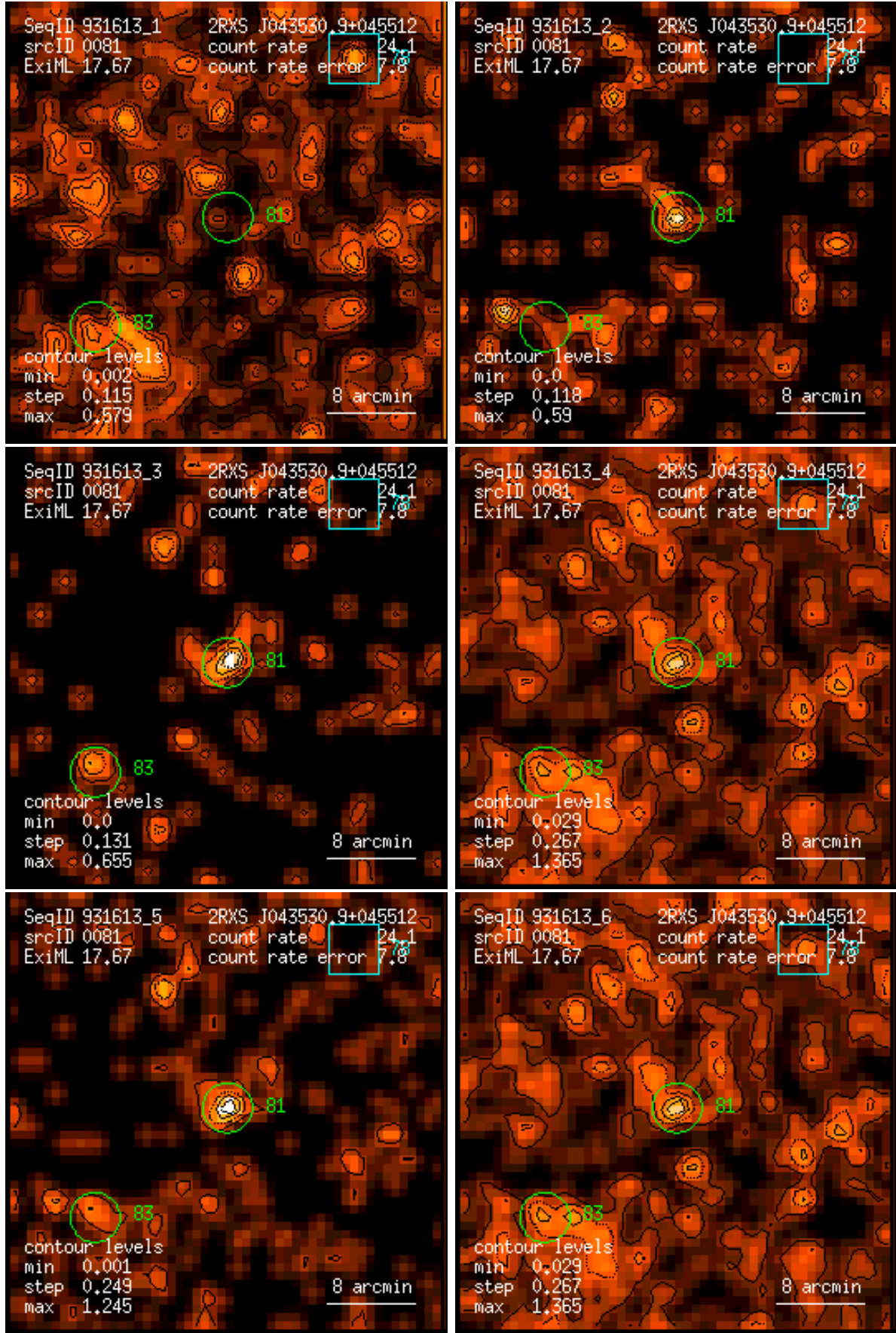
Figure 81: RASS 931613: detection 0081: band rate images, Gaussian filter: (1) PSPC channels 11 – 41, (2) 52 – 90, (3) 91 – 201, (4) 11 – 235, (5) 52 – 201, (6) 11 – 201. Broad band rates in counts/ks. Band rate contour levels in counts/ks/arcmin 2 .
