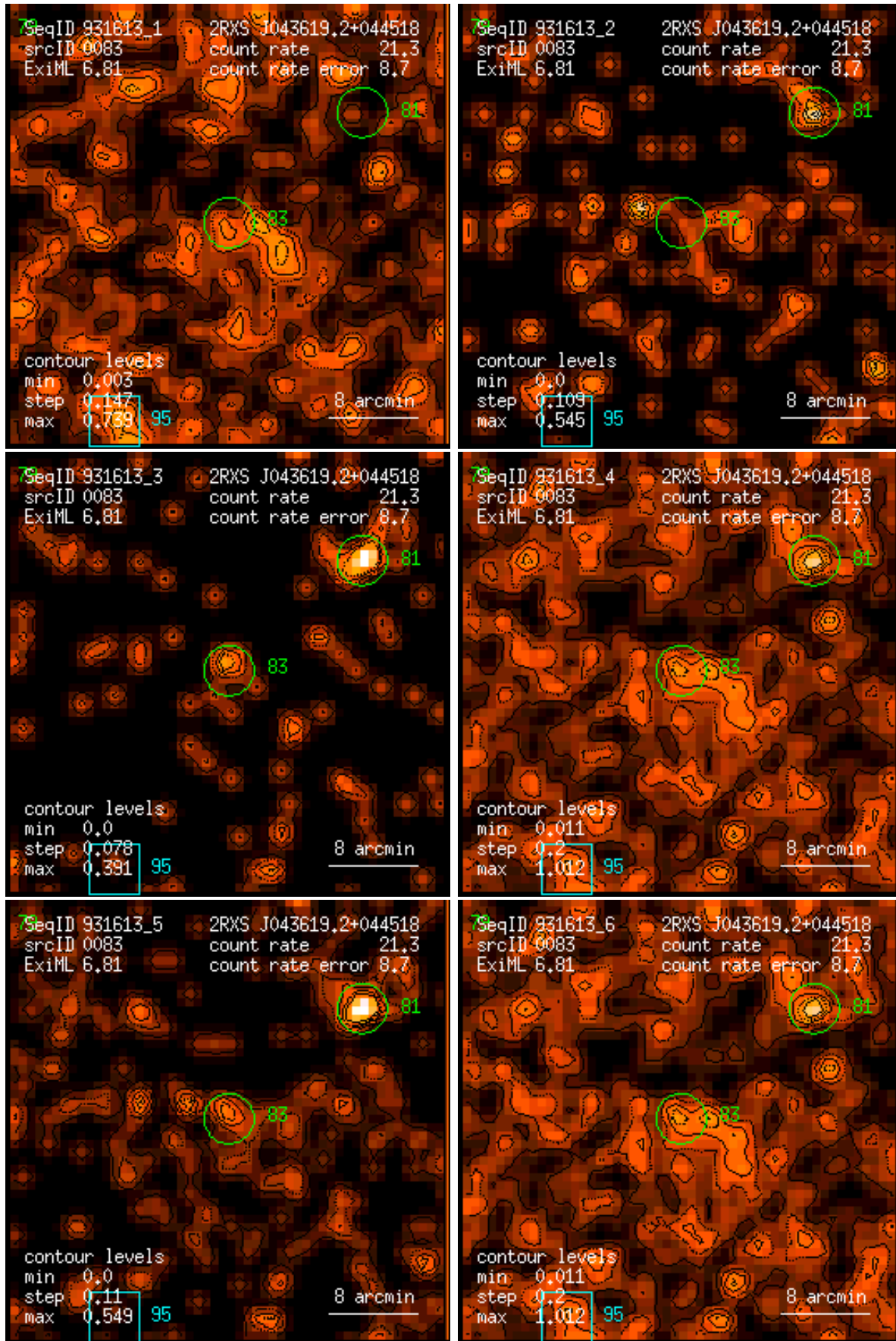
Figure 83: RASS 931613: detection 0083: band rate images, Gaussian filter: (1) PSPC channels 11 – 41, (2) 52 – 90, (3) 91 – 201, (4) 11 – 235, (5) 52 – 201, (6) 11 – 201. Broad band rates in counts/ks. Band rate contour levels in counts/ks/arcmin 2 .
