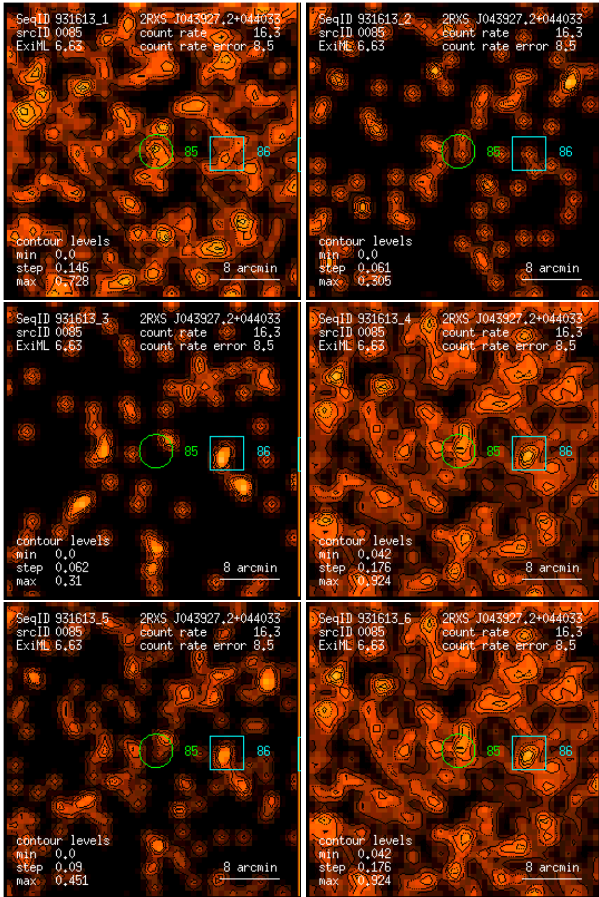
Figure 85: RASS 931613: detection 0085: band rate images, Gaussian filter: (1) PSPC channels 11 – 41, (2) 52 – 90, (3) 91 – 201, (4) 11 – 235, (5) 52 – 201, (6) 11 – 201. Broad band rates in counts/ks. Band rate contour levels in counts/ks/arcmin 2 .
