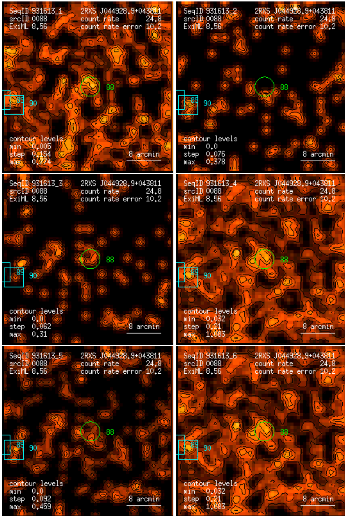
Figure 88: RASS 931613: detection 0088: band rate images, Gaussian filter: (1) PSPC channels 11 – 41, (2) 52 – 90, (3) 91 – 201, (4) 11 – 235, (5) 52 – 201, (6) 11 – 201. Broad band rates in counts/ks. Band rate contour levels in counts/ks/arcmin 2 .
