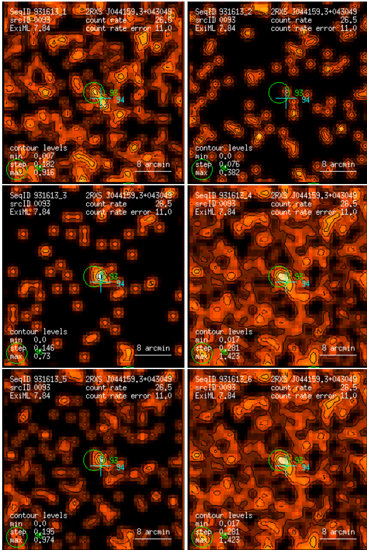
Figure 93: RASS 931613: detection 0093: band rate images, Gaussian filter: (1) PSPC channels 11 – 41, (2) 52 – 90, (3) 91 – 201, (4) 11 – 235, (5) 52 – 201, (6) 11 – 201. Broad band rates in counts/ks. Band rate contour levels in counts/ks/arcmin 2 .
