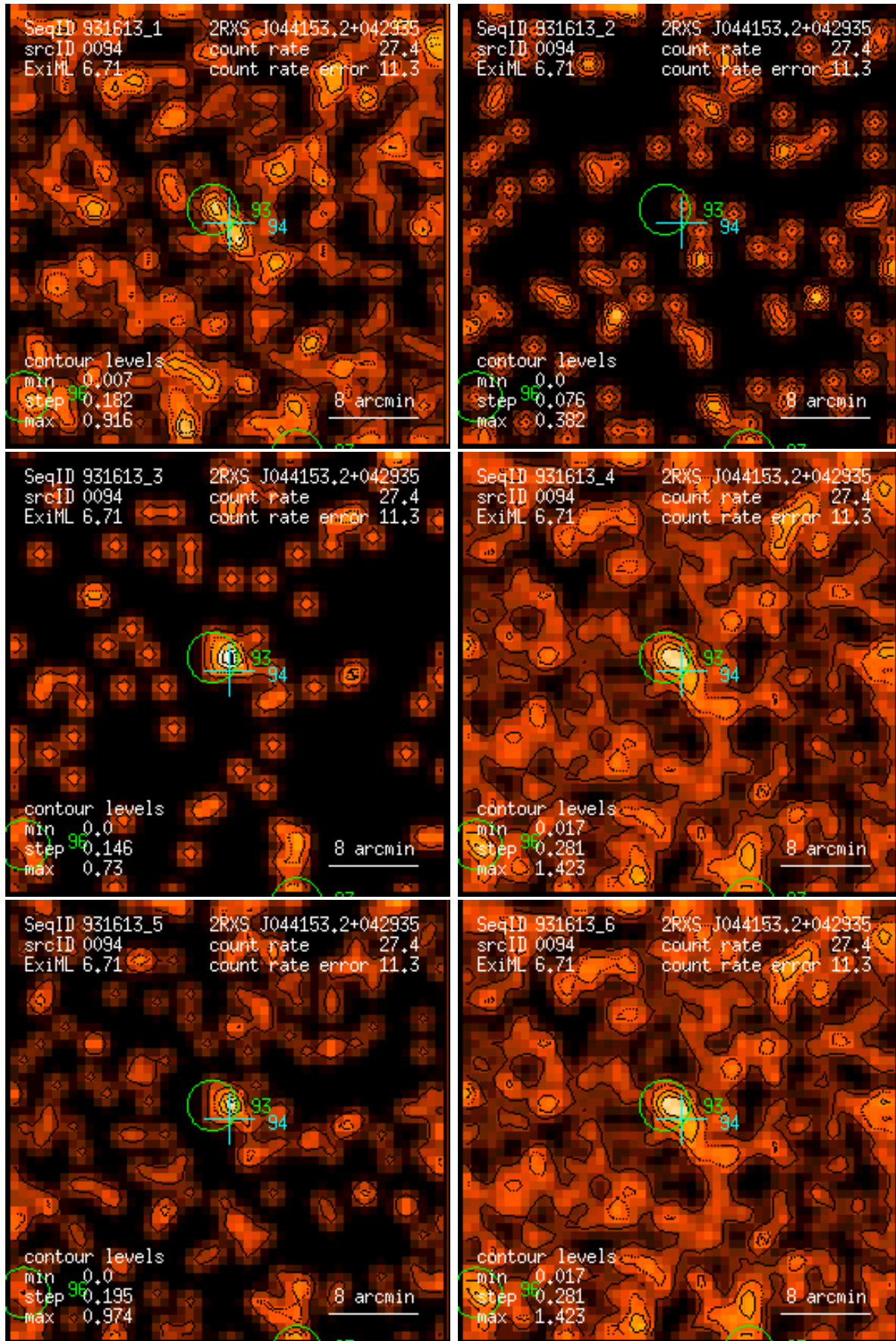
Figure 94: RASS 931613: detection 0094: band rate images, Gaussian filter: (1) PSPC channels 11 – 41, (2) 52 – 90, (3) 91 – 201, (4) 11 – 235, (5) 52 – 201, (6) 11 – 201. Broad band rates in counts/ks. Band rate contour levels in counts/ks/arcmin 2 .
