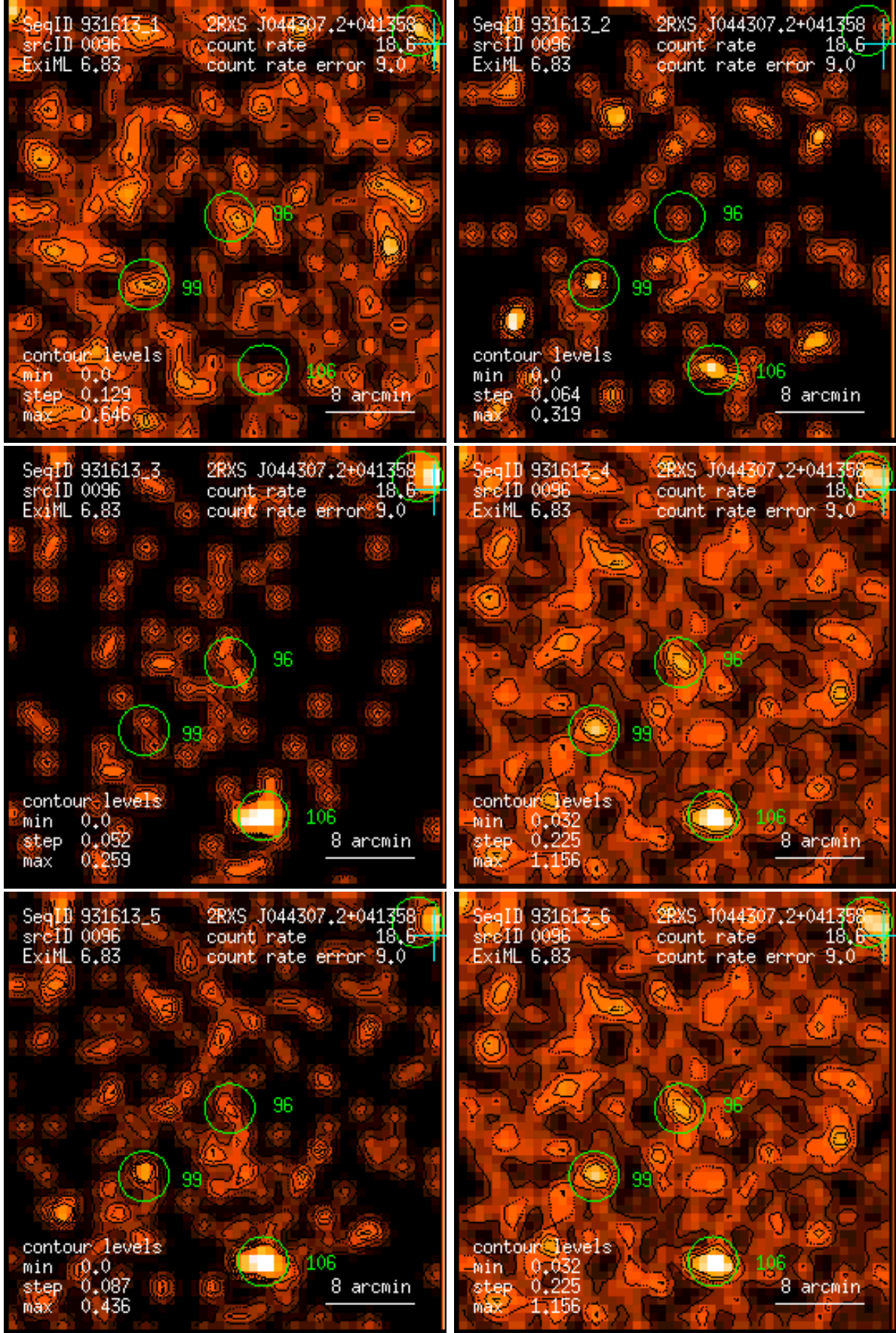
Figure 96: RASS 931613: detection 0096: band rate images, Gaussian filter: (1) PSPC channels 11 – 41, (2) 52 – 90, (3) 91 – 201, (4) 11 – 235, (5) 52 – 201, (6) 11 – 201. Broad band rates in counts/ks. Band rate contour levels in counts/ks/arcmin 2 .
