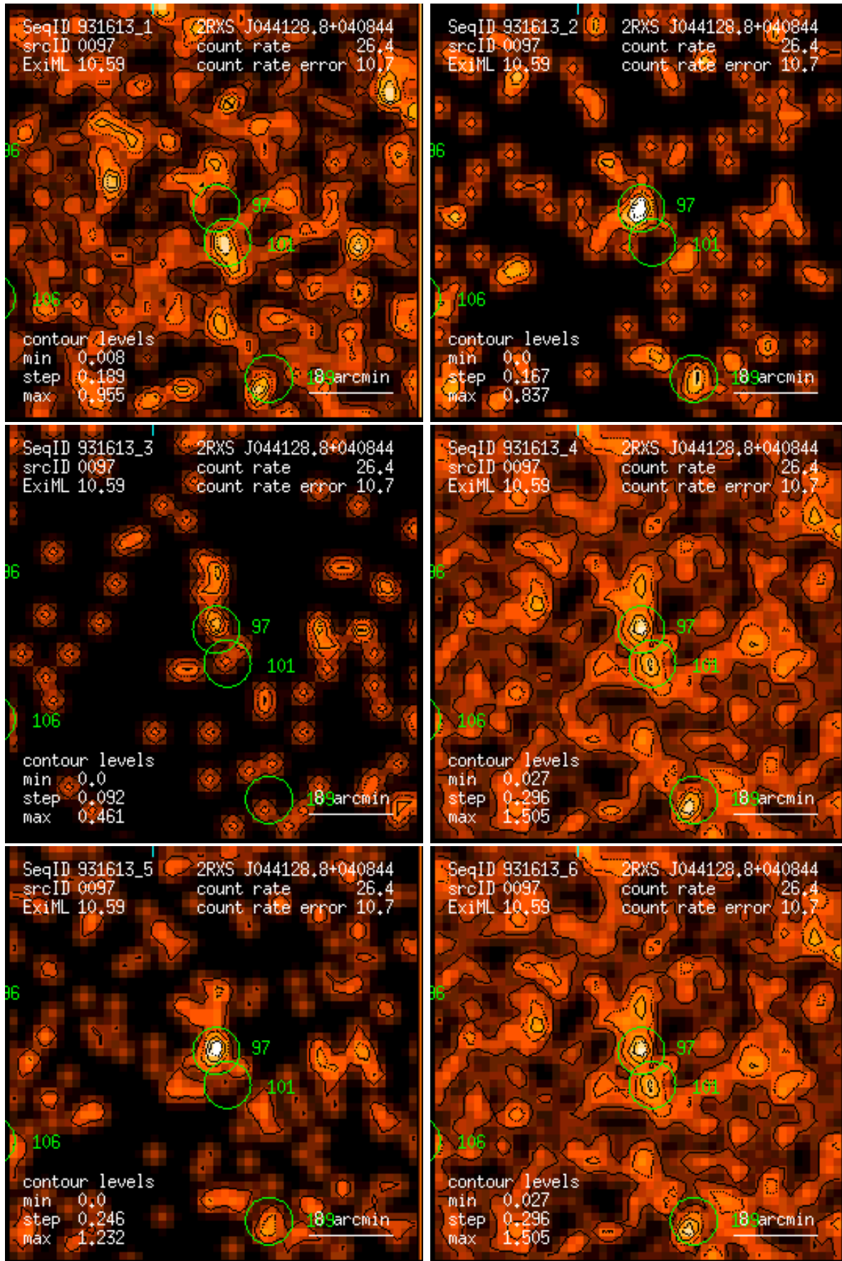
Figure 97: RASS 931613: detection 0097: band rate images, Gaussian filter: (1) PSPC channels 11 – 41, (2) 52 – 90, (3) 91 – 201, (4) 11 – 235, (5) 52 – 201, (6) 11 – 201. Broad band rates in counts/ks. Band rate contour levels in counts/ks/arcmin 2 .
