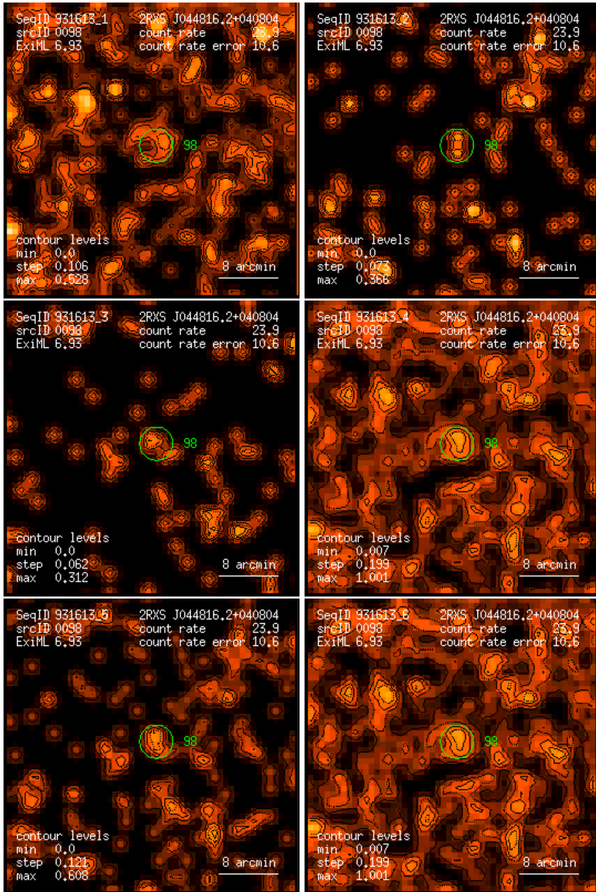
Figure 98: RASS 931613: detection 0098: band rate images, Gaussian filter: (1) PSPC channels 11 – 41, (2) 52 – 90, (3) 91 – 201, (4) 11 – 235, (5) 52 – 201, (6) 11 – 201. Broad band rates in counts/ks. Band rate contour levels in counts/ks/arcmin 2 .
